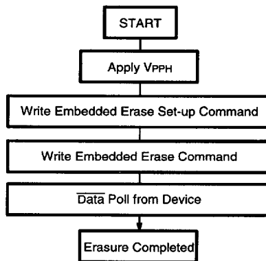
Figure 5. Embedded Erase Algorithm
