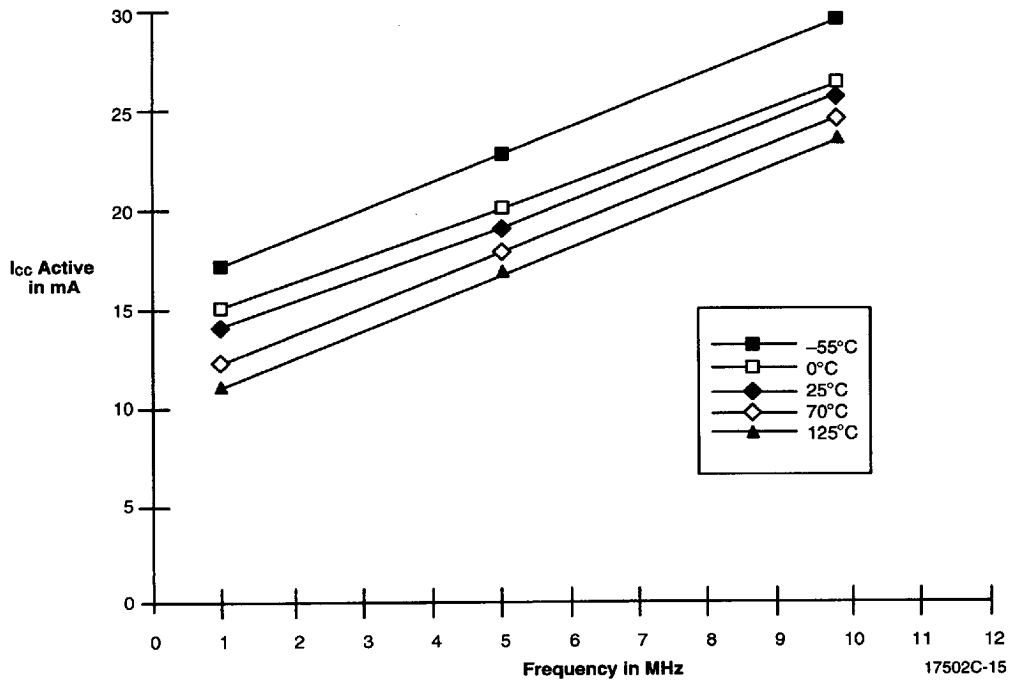
Figure 9. Am28F020A - Average Icc Active vs. Frequency V_{CC} = 5.5 \text{ V} , Addressing Pattern = Minmax Data Pattern = Checkerboard
