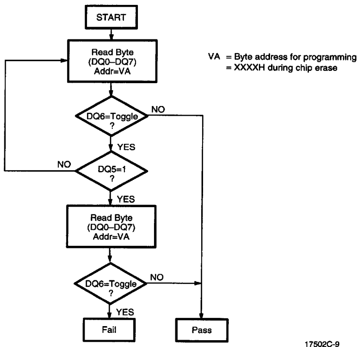
Figure 7b. Toggle Bit Algorithm
