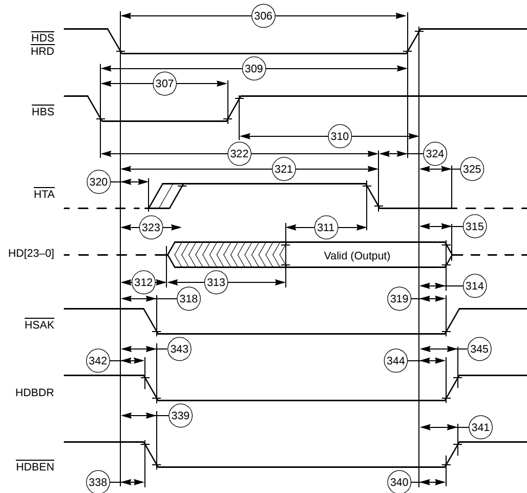
Figure 2-32. Read Timing
