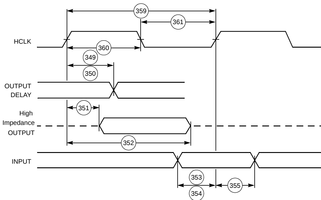
Figure 2-36. PCI Timing
