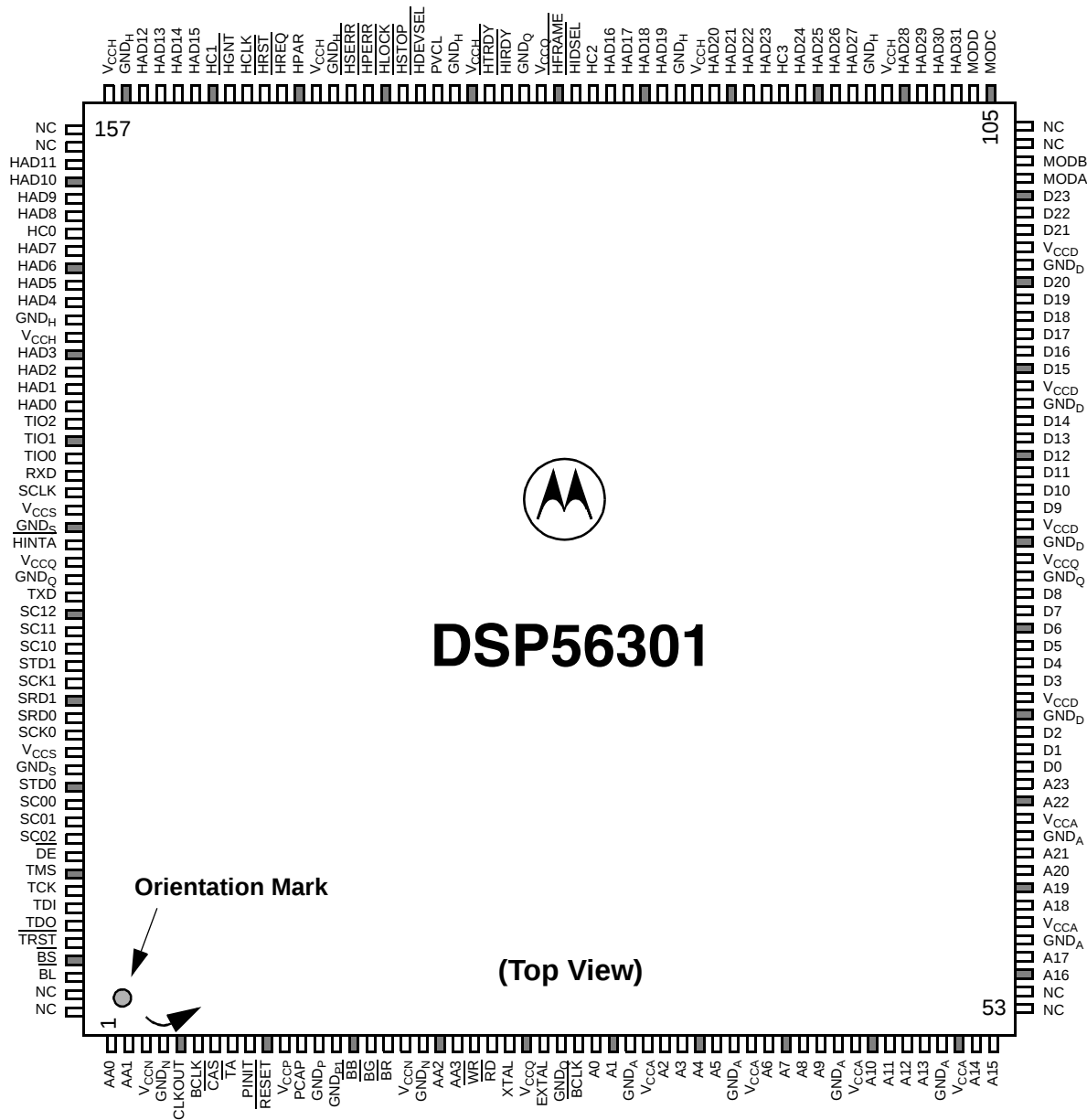
Figure 3-1. DSP56301 Thin Quad Flat Pack (TQFP), Top View
