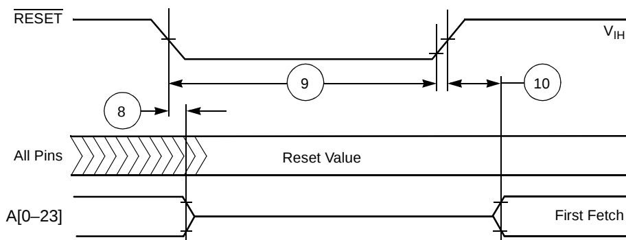
Figure 2-3. Reset Timing
