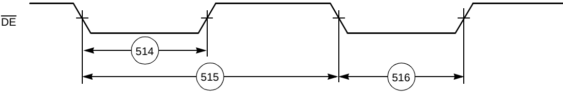
Figure 2-50. OnCE—Debug Request
