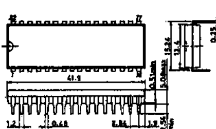
SANYO: DIP32
