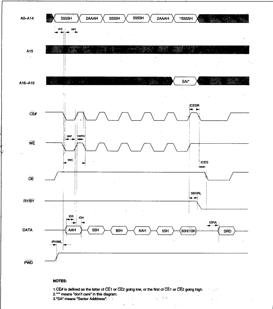
Figure 9. AUTOMATIC SECTOR/CHIP ERASE TIMING WAVEFORMS
