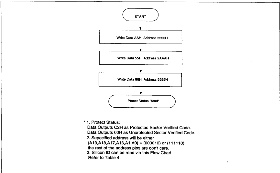
Figure 12. VERIFY SECTOR PROTECT FLOW CHART
