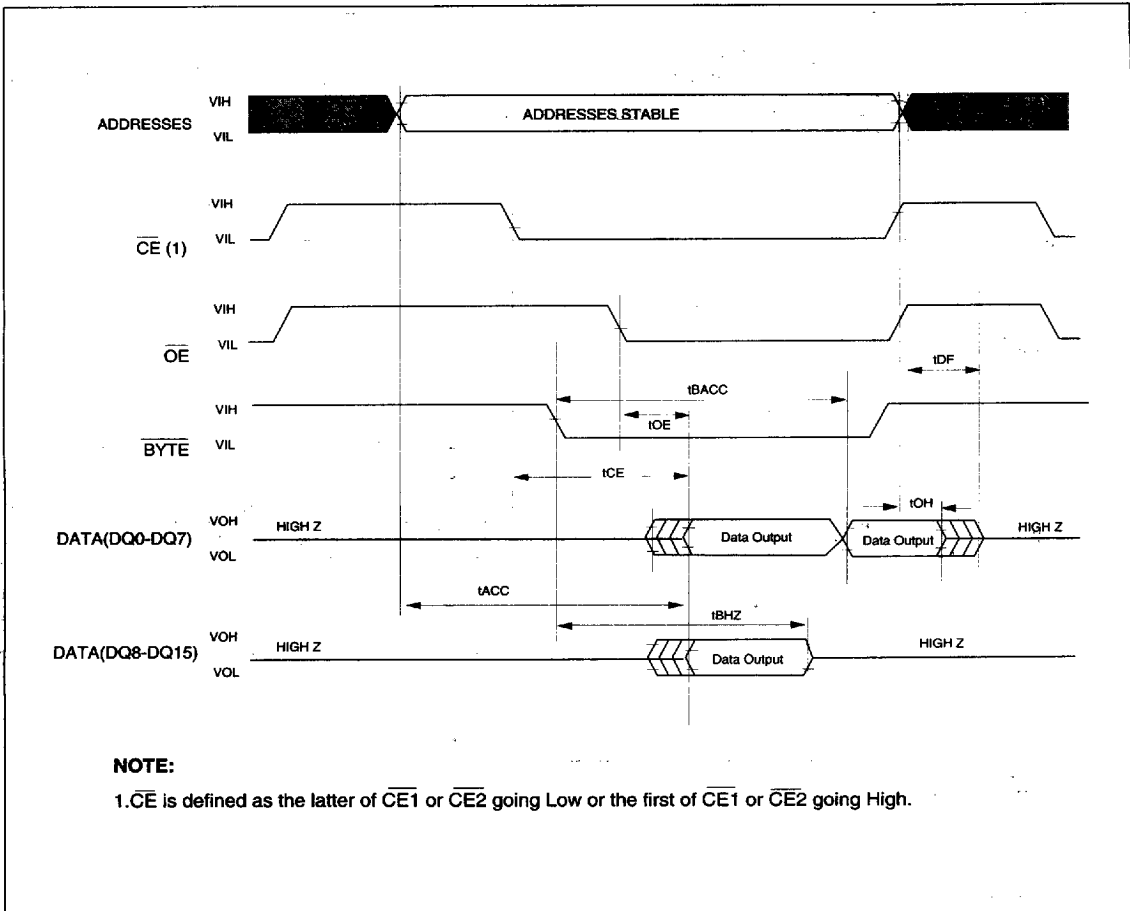
Figure 6. BYTE TIMING WAVEFORMS
