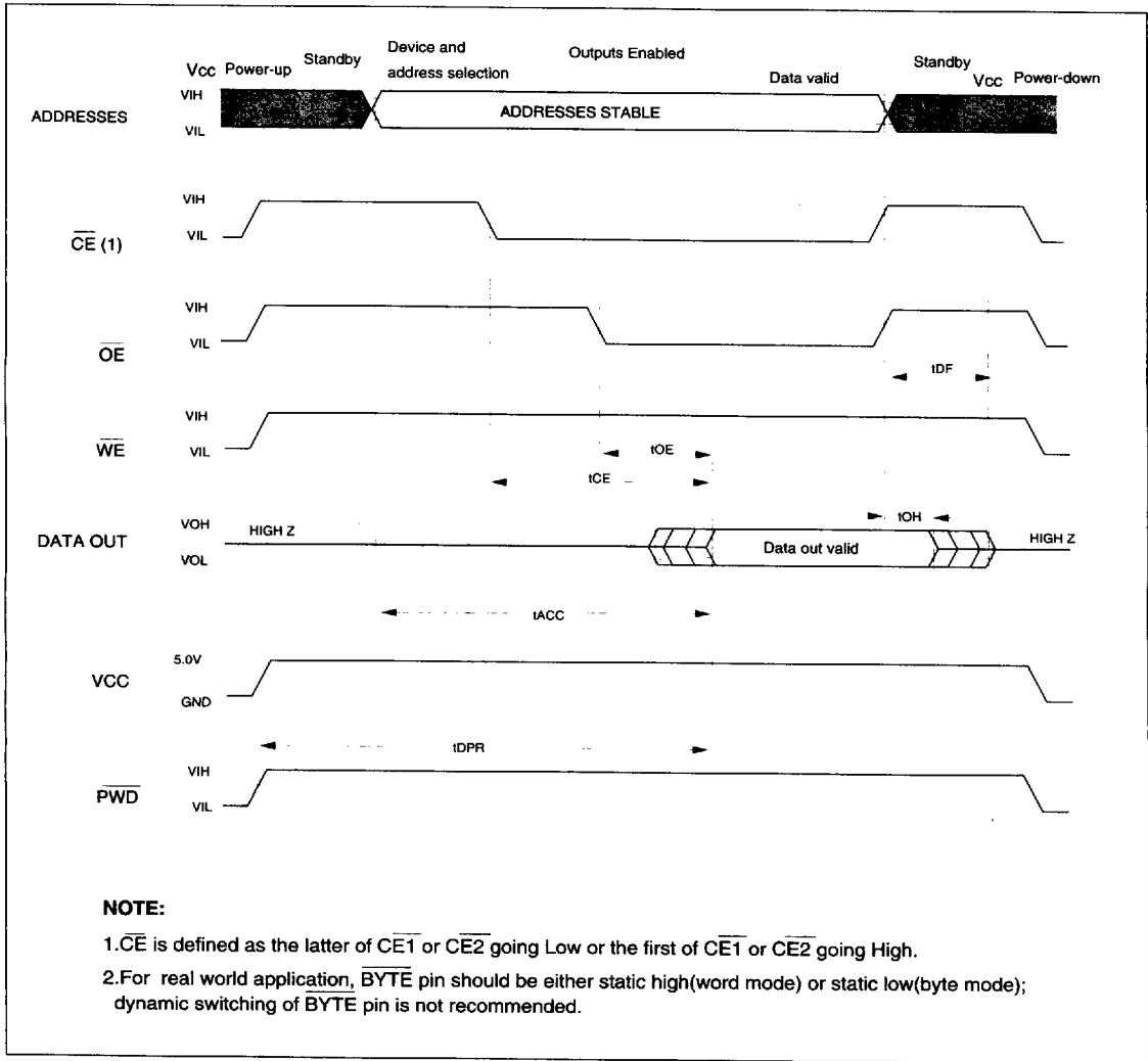
Figure 5. READ TIMING WAVEFORMS
