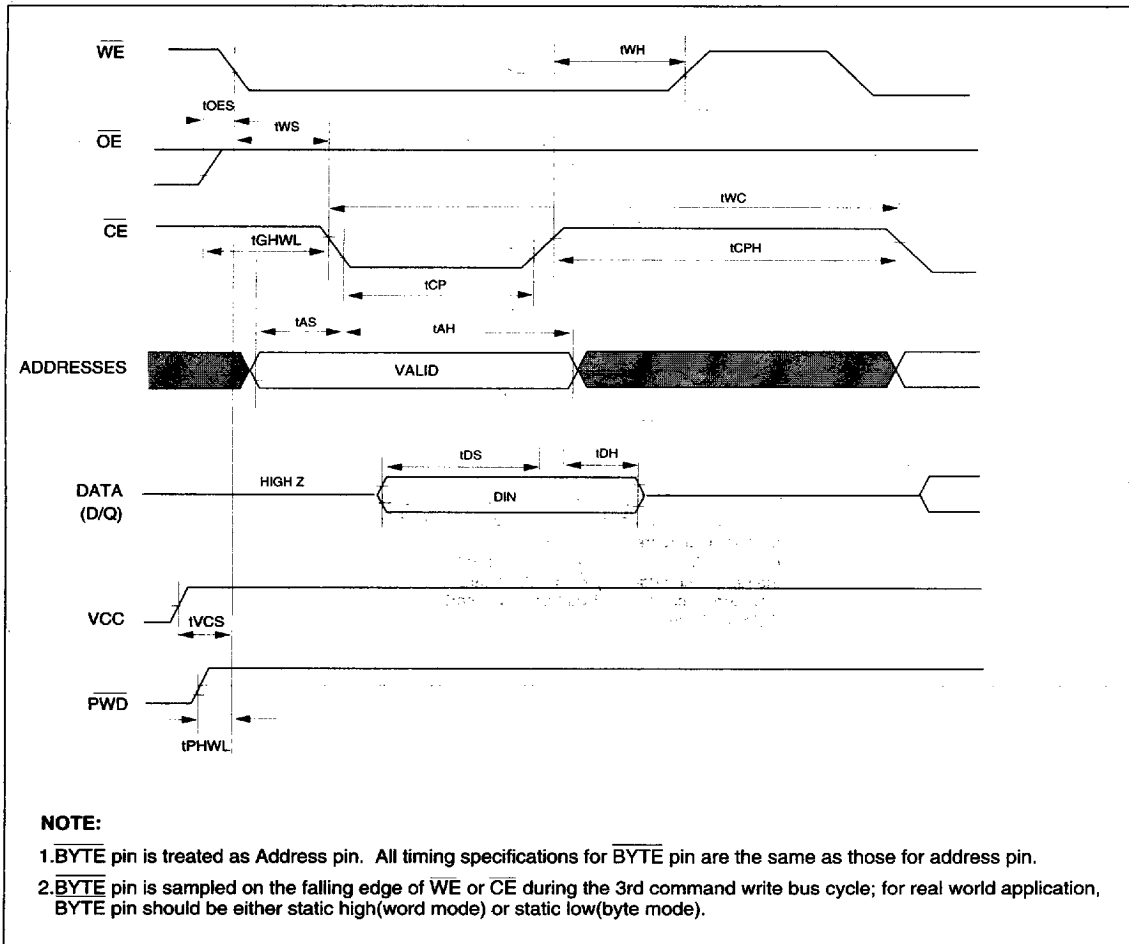
Figure 13. COMMAND WRITE TIMING WAVEFORMS(Alternate \overline{CE} Controlled)
