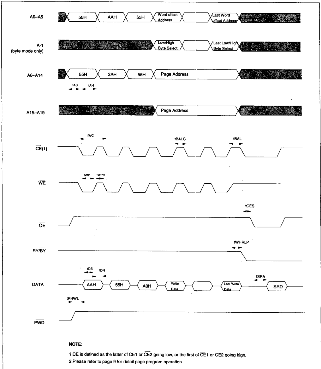
Figure 8. AUTOMATIC PAGE PROGRAM TIMING WAVEFORMS
