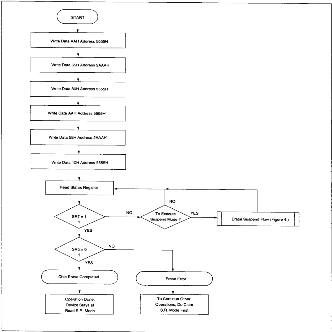
Figure 2. AUTOMATIC CHIP ERASE FLOW CHART
