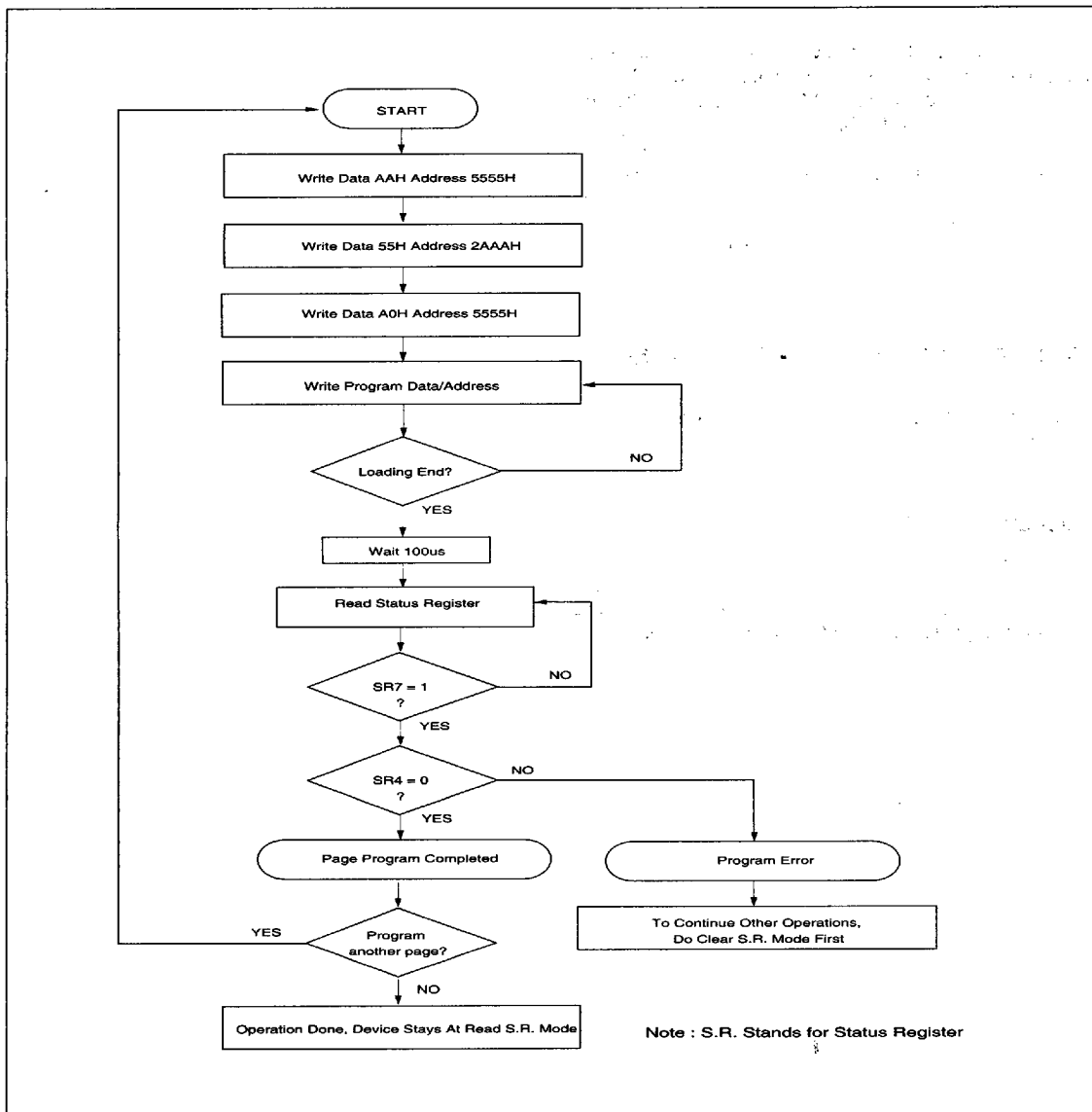
Figure 1. AUTOMATIC PAGE PROGRAM FLOW CHART
