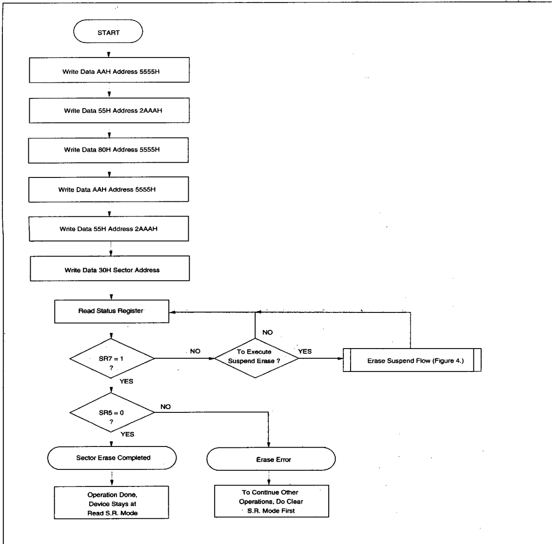
Figure 3. AUTOMATIC SECTOR ERASE FLOW CHART
