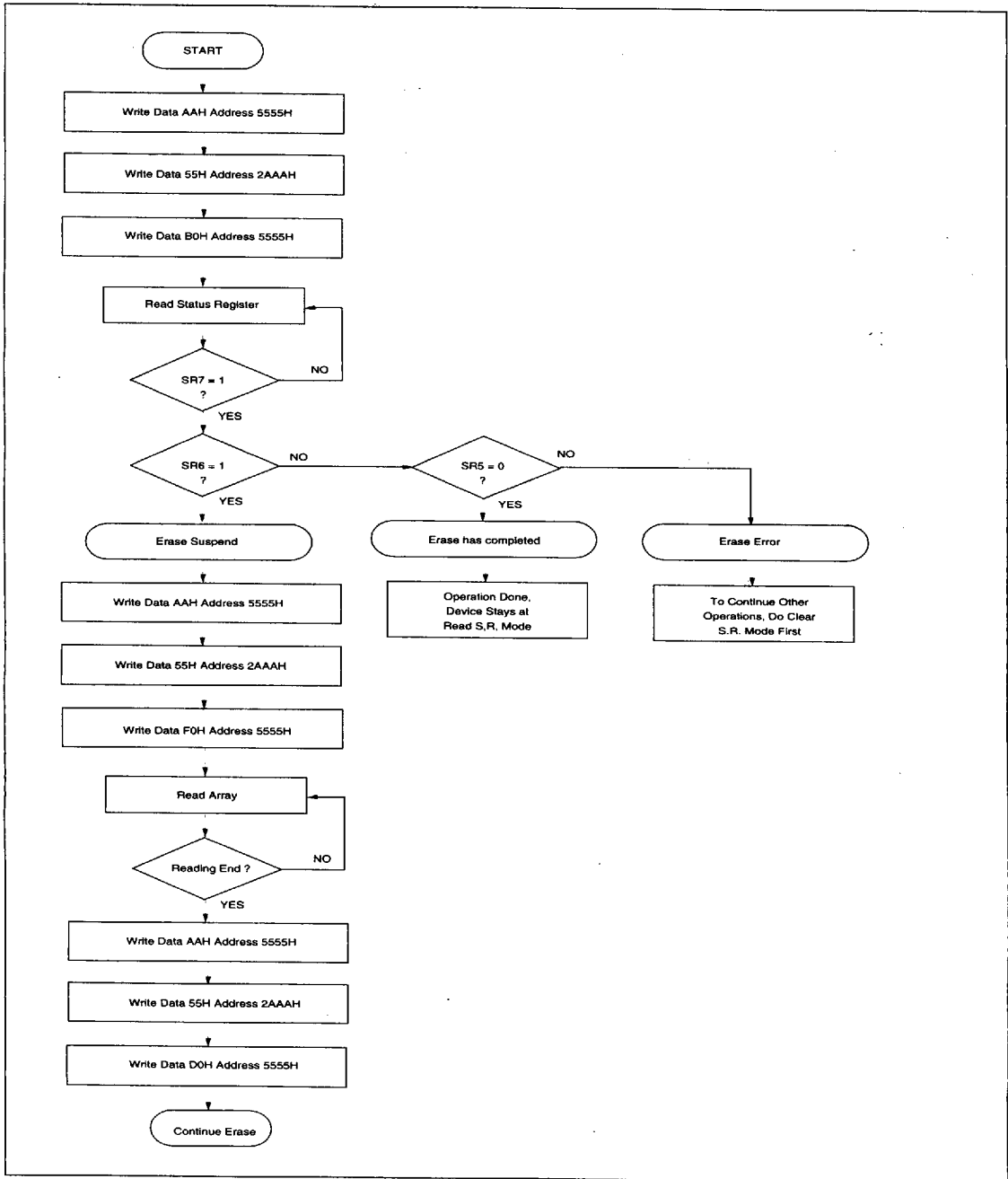
Figure 4. ERASE SUSPEND/ERASE RESUME FLOW CHART
