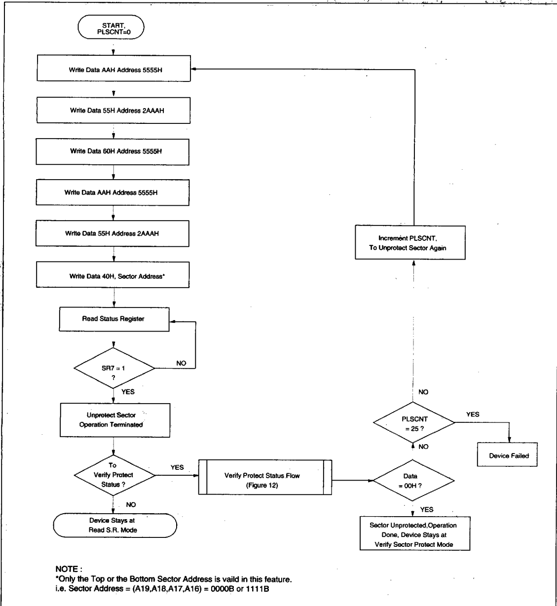
Figure 11. SECTOR UNPROTECT ALGORITHM
