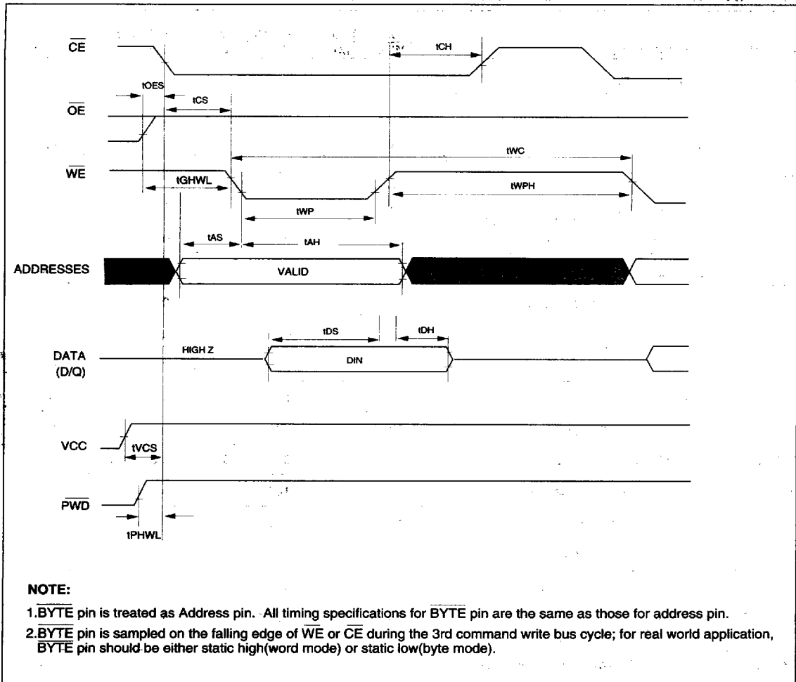
Figure 7. COMMAND WRITE TIMING WAVEFORMS
