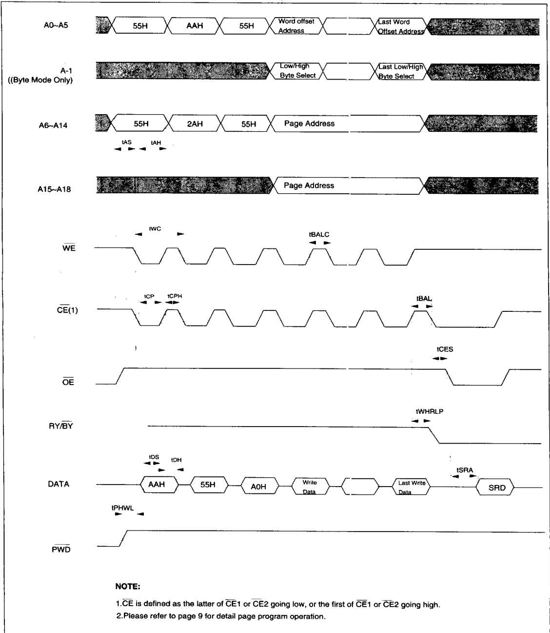
Figure 14. AUTOMATIC PAGE PROGRAM TIMING WAVEFORM(Alternate \overline{CE} Controlled)
