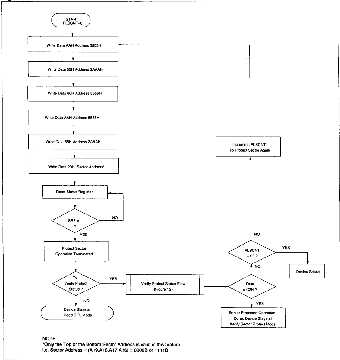
Figure 10. SECTOR PROTECTION ALGORITHM
