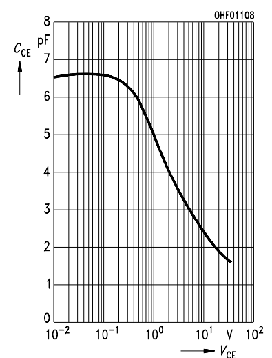
Collector-emitter capacitance
