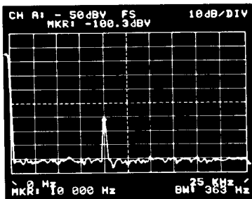
Figure 16. Multiplying Feedthrough
