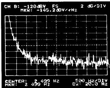
Figure 17. Lowband Noise Spectrum
