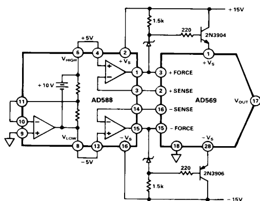
d. AD588 Produces References and Supply Voltages
