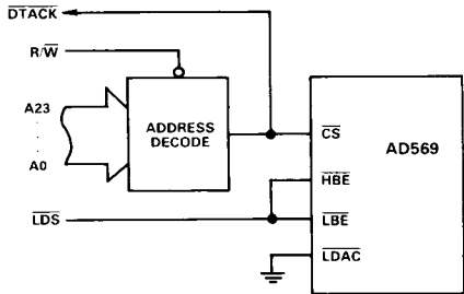
Figure 19. AD569/68000 Interface
