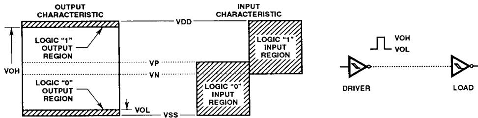
FIGURE 18. INPUT AND OUTPUT CHARACTERISTICS
