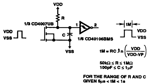
FIGURE 15. MONOSTABLE MULTIVIBRATOR
