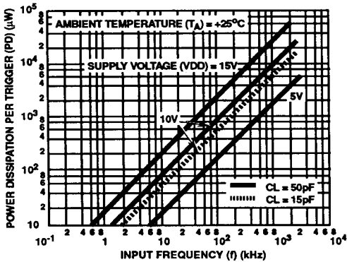
FIGURE 10. TYPICAL POWER DISSIPATION PER TRIGGER AS A FUNCTION OF INPUT FREQUENCY
