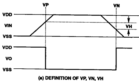
FIGURE 17. HYSTERESIS DEFINITION, CHARACTERISTICS, AND TEST SETUP
