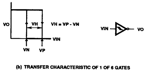
FIGURE 17. HYSTERESIS DEFINITION, CHARACTERISTICS, AND TEST SETUP
