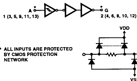
FIGURE 1. 1 OF 6 SCHMITT TRIGGERS
