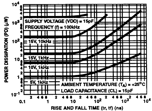
FIGURE 13. TYPICAL POWER DISSIPATION AS A FUNCTION OF RISE AND FALL TIMES
