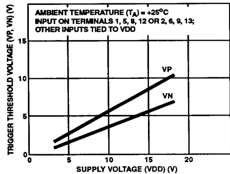
FIGURE 11. TYPICAL TRIGGER THRESHOLD VOLTAGE AS A FUNCTION OF SUPPLY VOLTAGE
