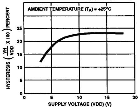
FIGURE 12. TYPICAL PERCENT HYSTERESIS AS A FUNCTION OF SUPPLY VOLTAGE
