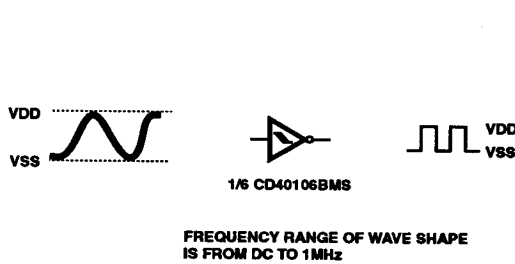
FIGURE 14. WAVE SHAPER
