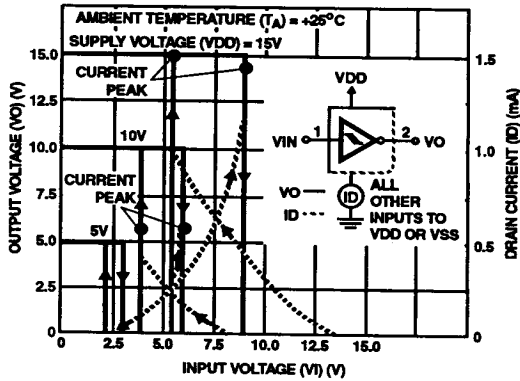
FIGURE 6. TYPICAL CURRENT AND VOLTAGE TRANSFER CHARACTERISTICS
