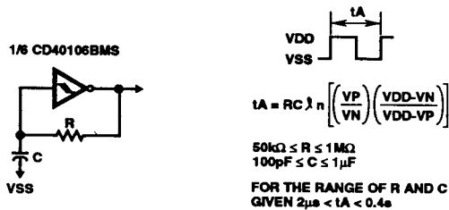
FIGURE 16. ASTABLE MULTIVIBRATOR
