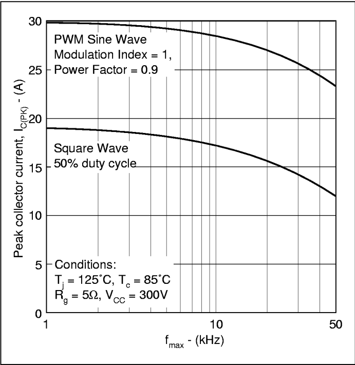
Fig.18 Three Phase PWM inverter operating frequency
