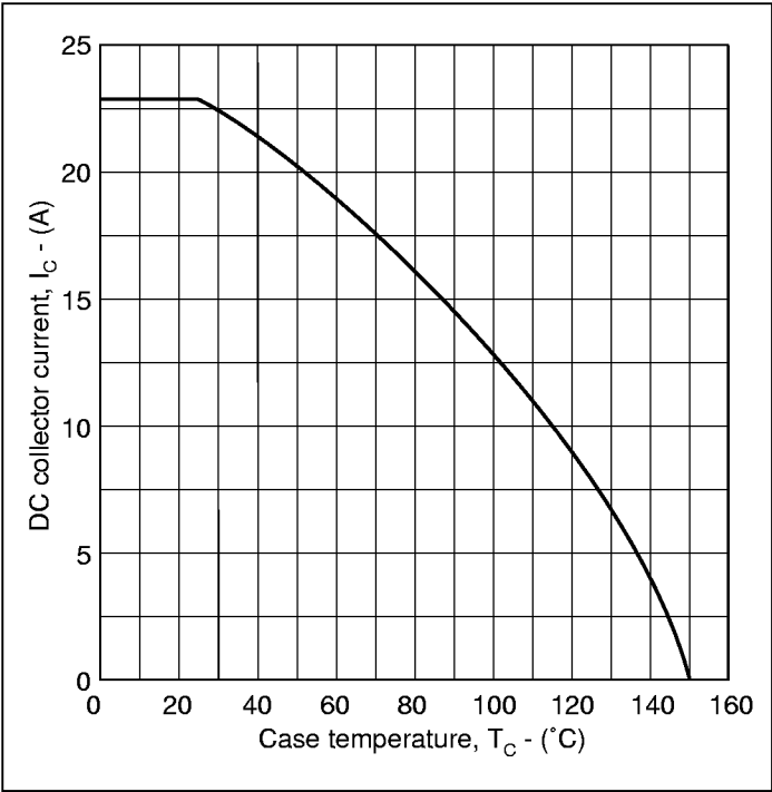
Fig.19 DC current rating vs case temperature
