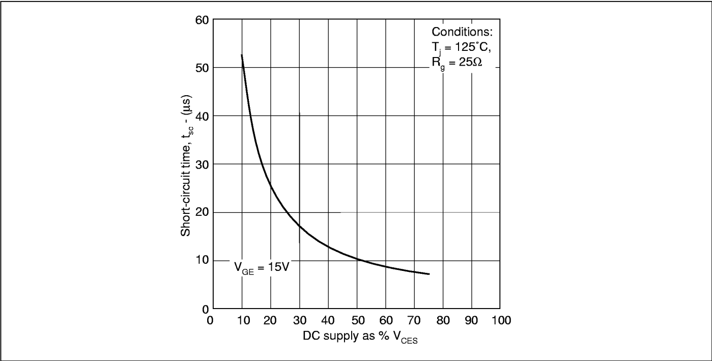
Fig.20 Short circuit withstand
