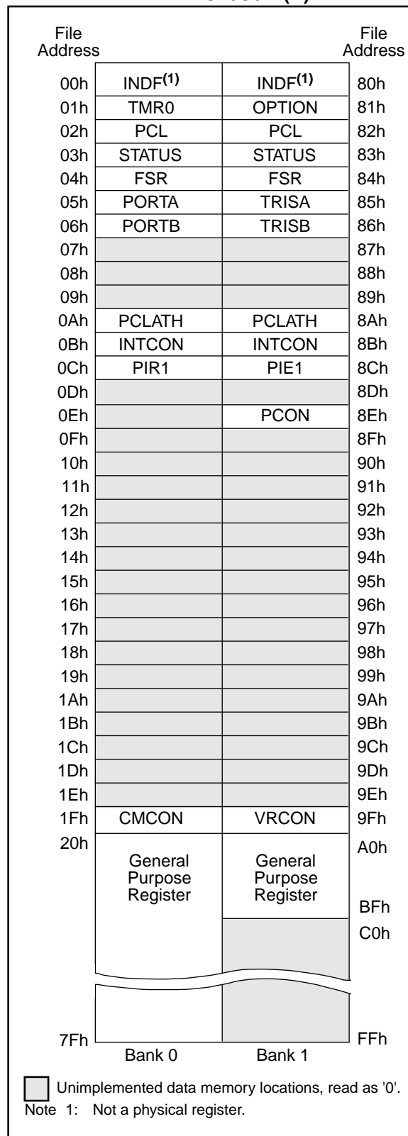
FIGURE 4-5: DATA MEMORY MAP FOR THE PIC16C622(A)
