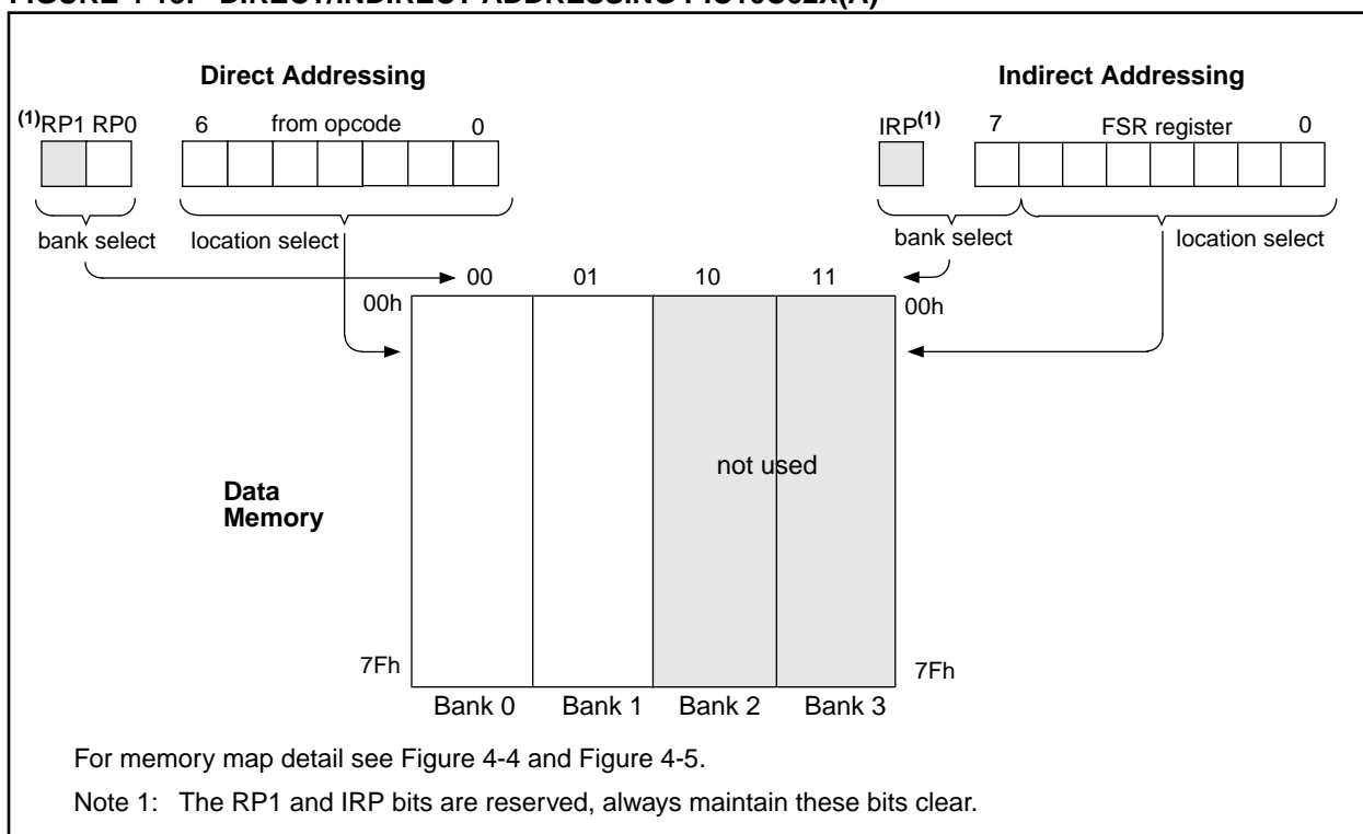
FIGURE 4-13: DIRECT/INDIRECT ADDRESSING PIC16C62X(A)
