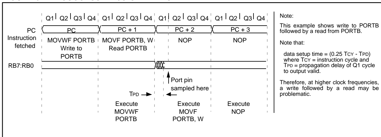
FIGURE 5-7: SUCCESSIVE I/O OPERATION
