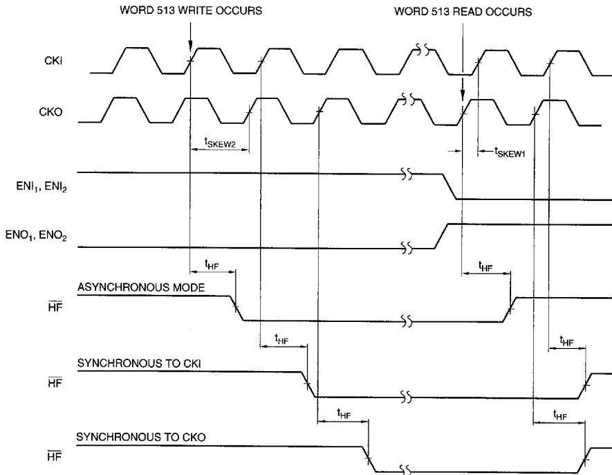
FIGURE 14. HALF-FULL FLAG: SYNCHRONOUS AND ASYNCHRONOUS MODES
