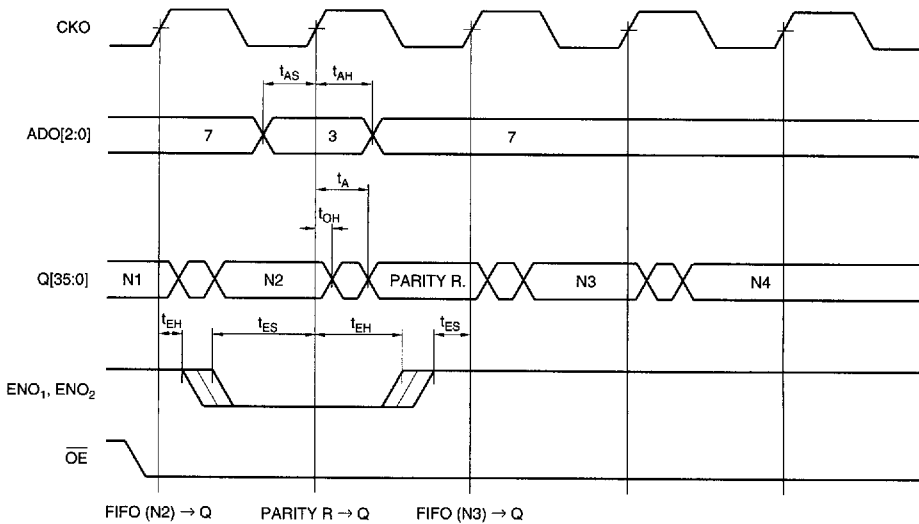
FIGURE 18. READ RESOURCE REGISTER
