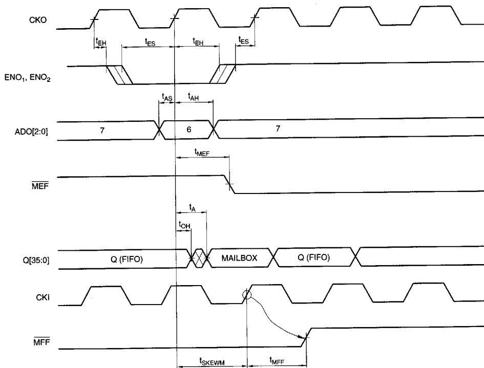
FIGURE 23. MAILBOX REGISTER
