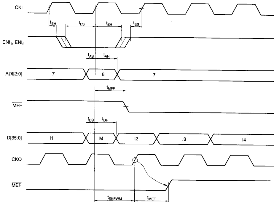
FIGURE 24. MAILBOX WRITE
