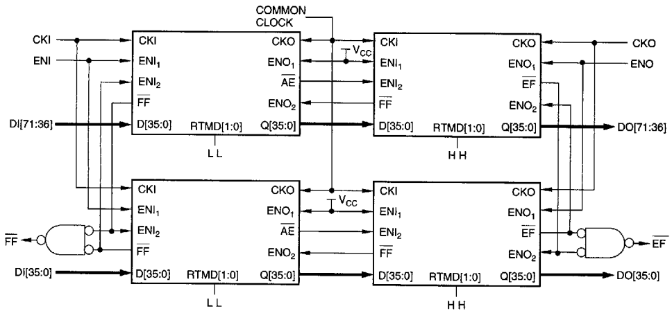
C. "Two-Dimension" Pipelined Cascading Mode
