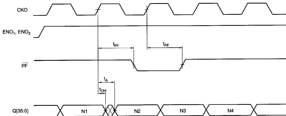
FIGURE 16. PARITY FLAG
