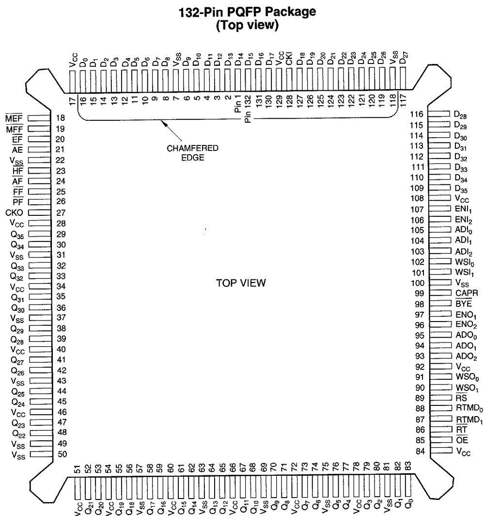
FIGURE 3. PINOUTS
