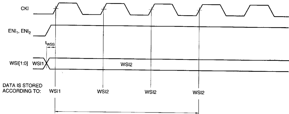
FIGURE 21. WSI[1:0] TIMING
