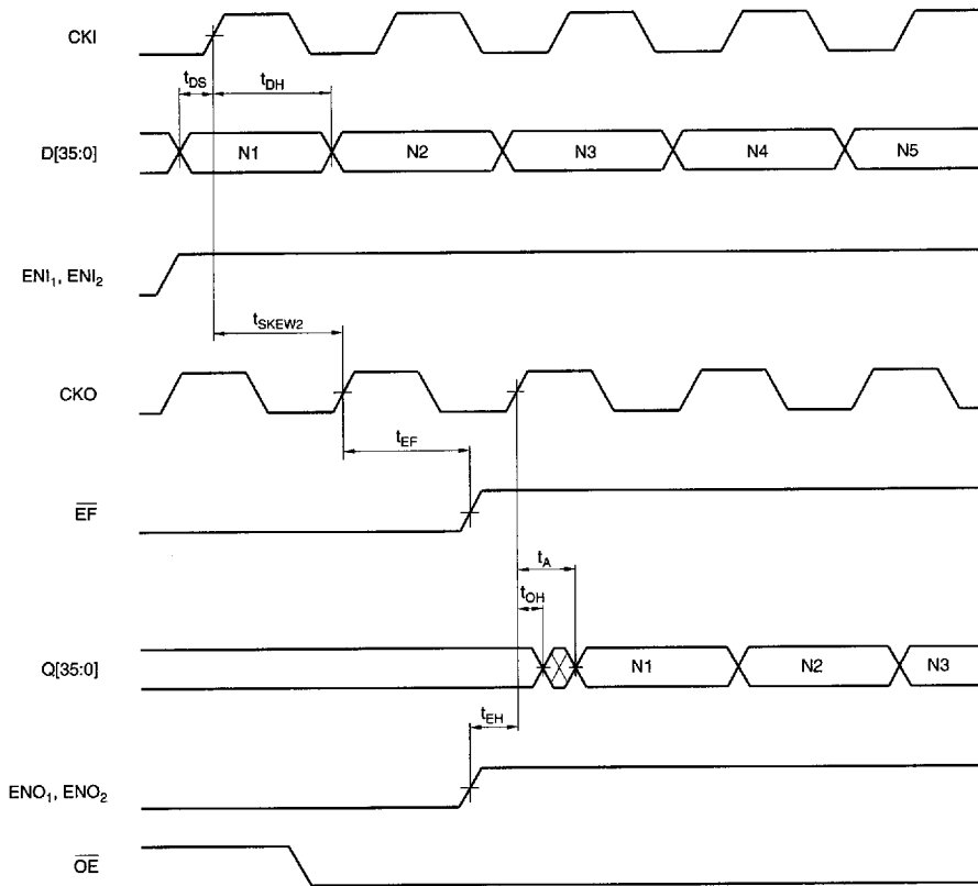
FIGURE 15. FIRST WORD LATENCY
