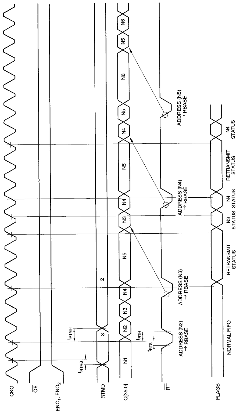
FIGURE 25. RETRANSMIT USING RETRANSMIT AND MARK MODE
