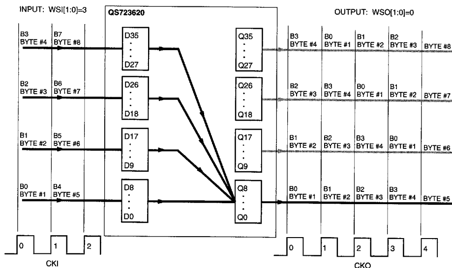
FIGURE 5. EXAMPLE OF 36-TO-9 BUS FUNNELING
