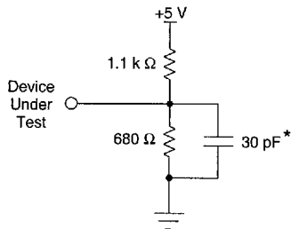
FIGURE 9. OUTPUT LOAD CIRCUIT
