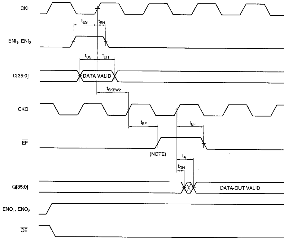
FIGURE 12. EMPTY FLAG TIMING
