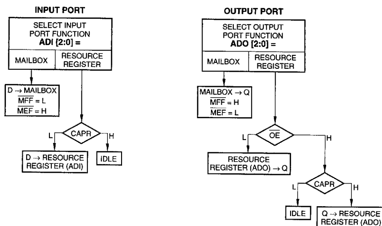
FIGURE 4. RESOURCE REGISTERS, READ AND WRITE
