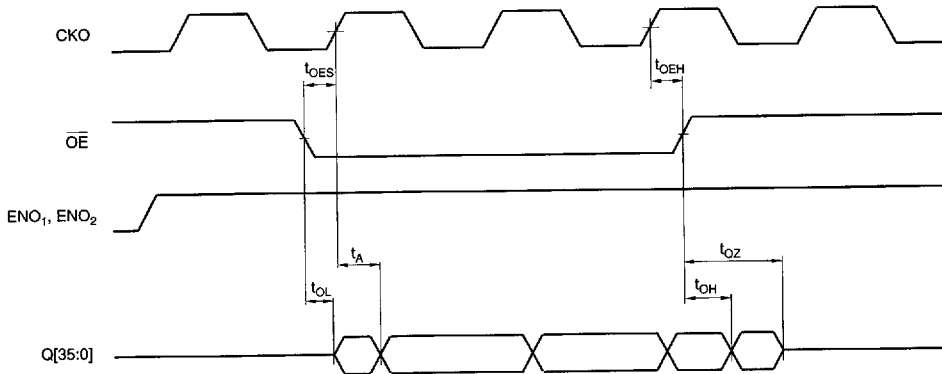
FIGURE 27. \overline{OE} WHEN BIT 6 OF THE CONTROL REGISTER IS HIGH
