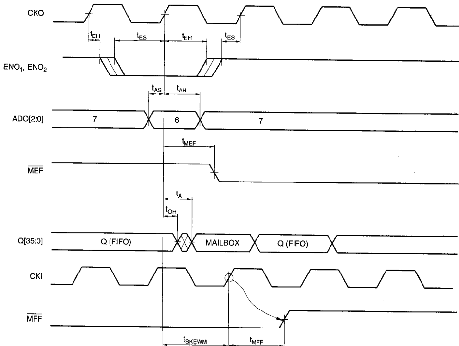
FIGURE 22. WSO[1:0] TIMING
