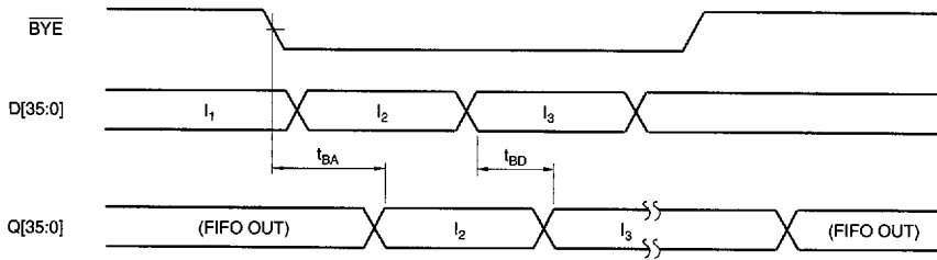
FIGURE 17. BYPASS
