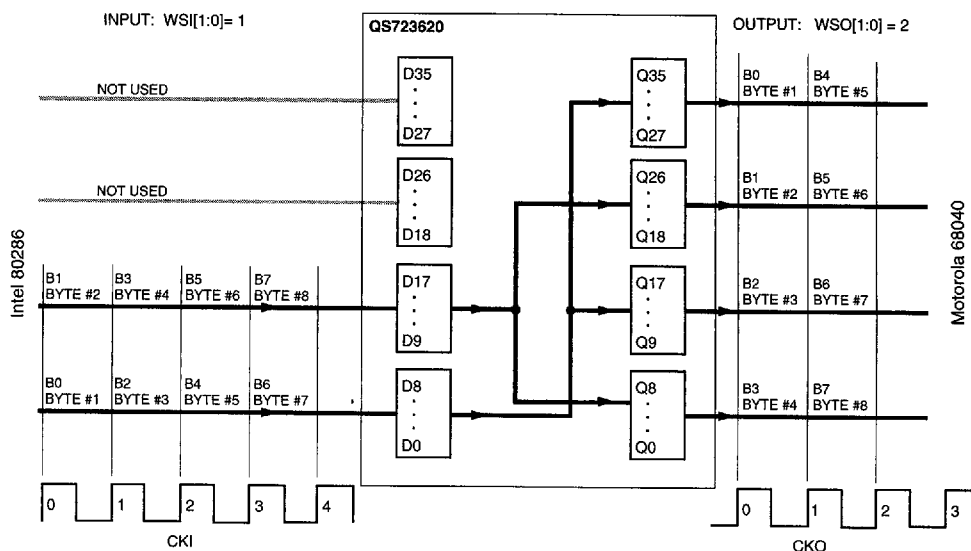
FIGURE 6. EXAMPLE OF 18-TO-36 BUS DEFUNNELING WITH BYTE-ORDER-REVERSAL
