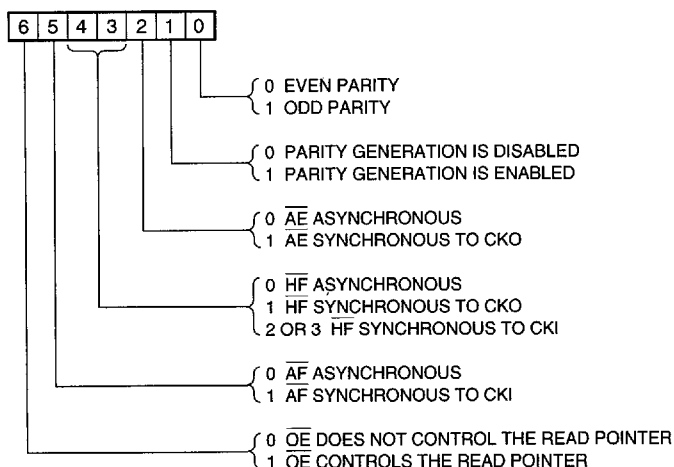
FIGURE 7. QS723620 CONTROL REGISTER
