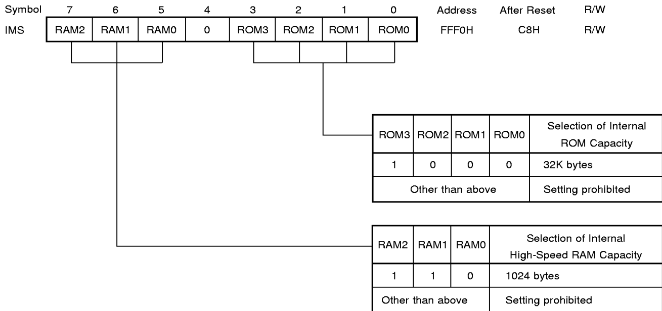
Figure 3-1. Memory Size Switching Register Format
