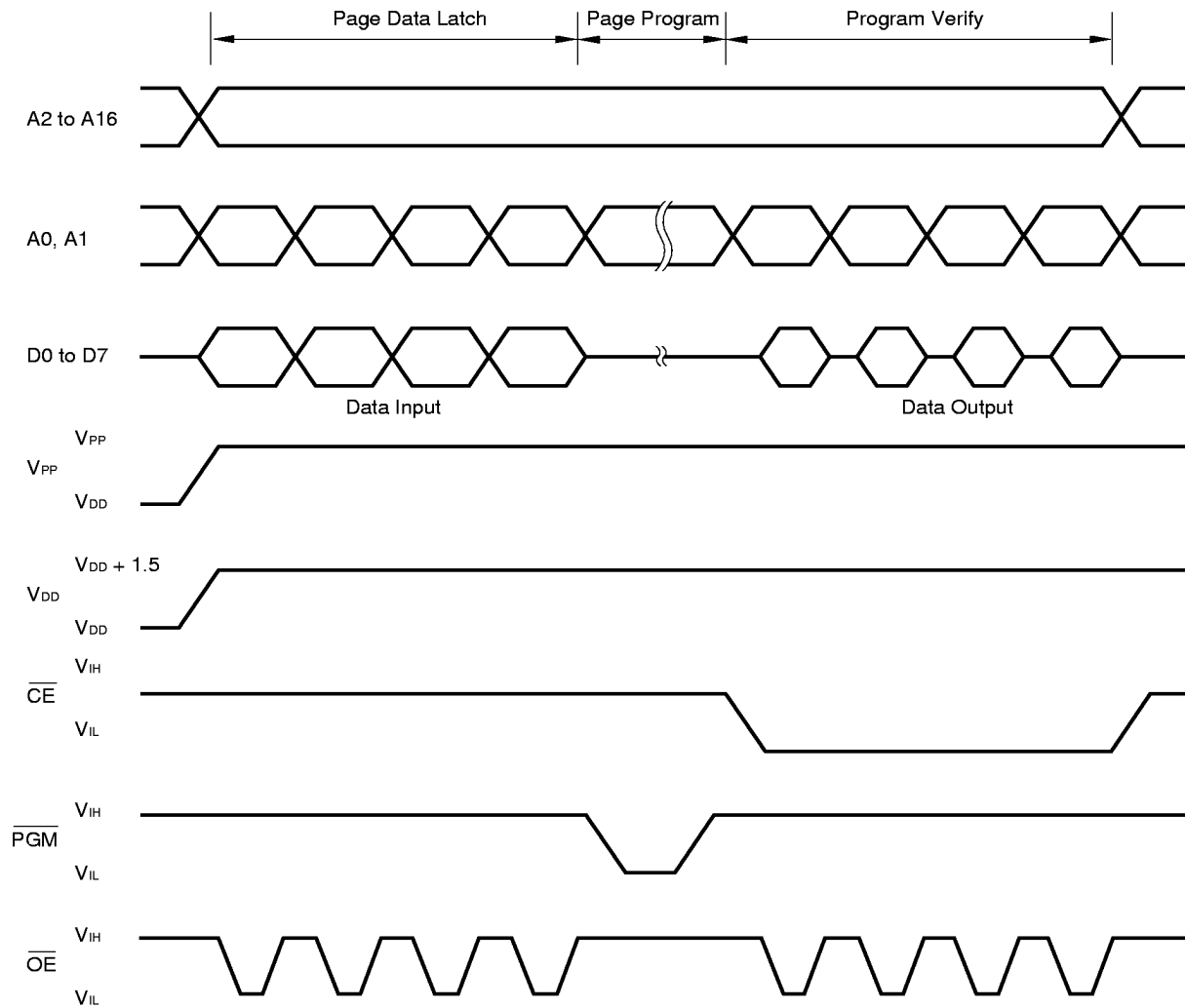
Figure 4-2. Page Program Mode Timing
