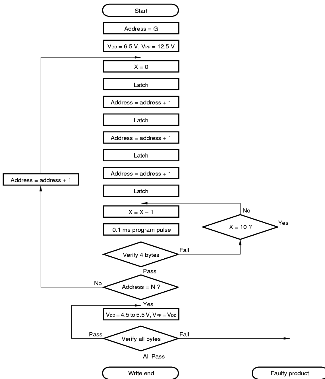
Figure 4-1. Page Program Mode Flow Chart
