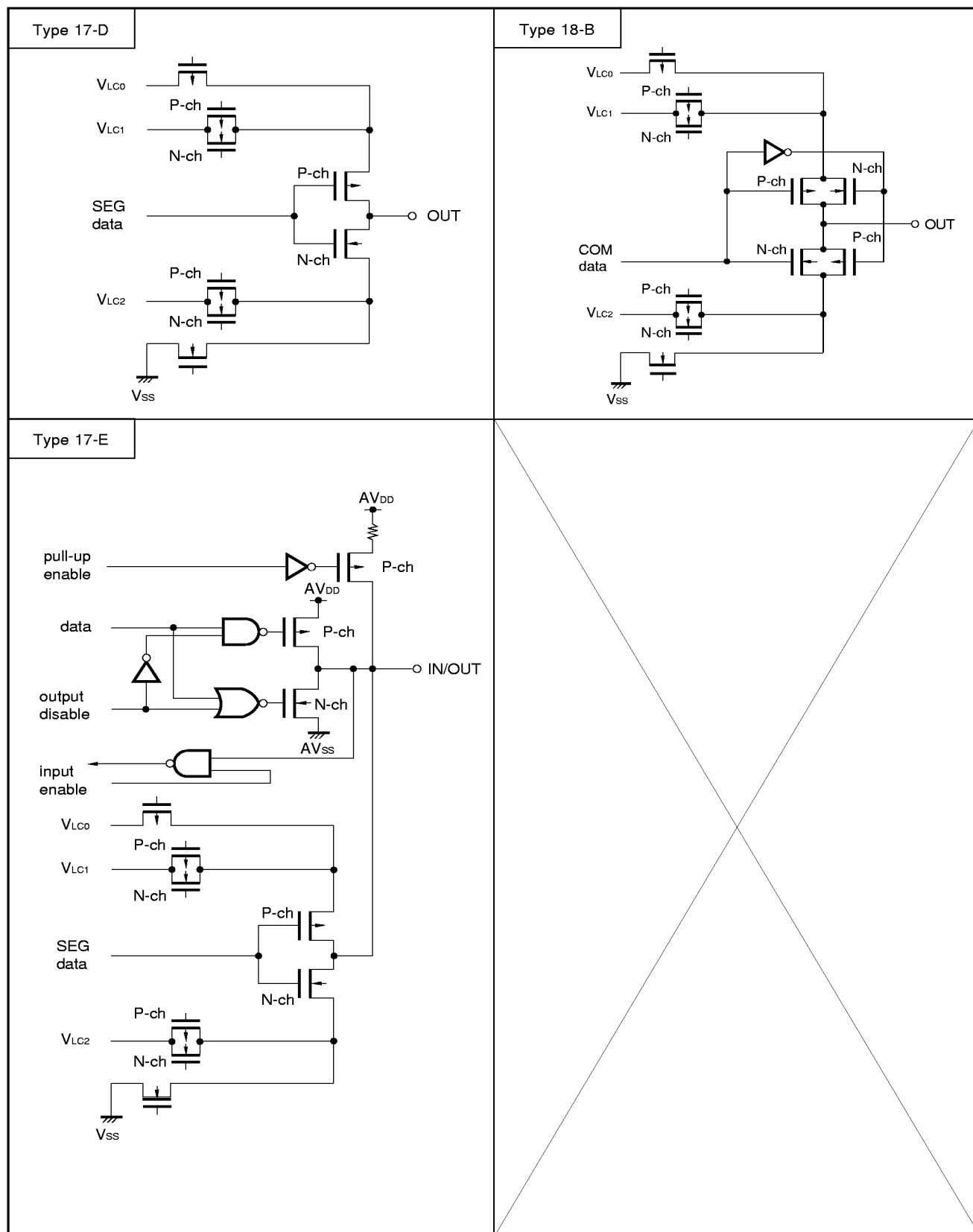
Figure 2-1. List of Pin Input/Output Circuits (2/2)
