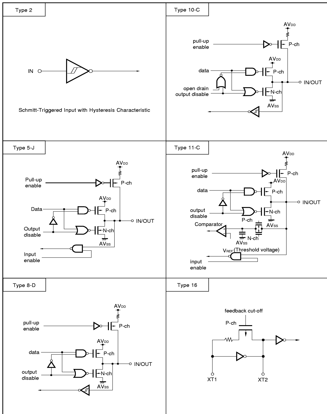
Figure 2-1. List of Pin Input/Output Circuits (1/2)
