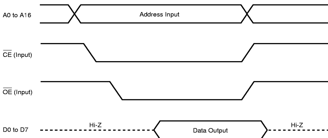
Figure 4-5. PROM Read Timings
