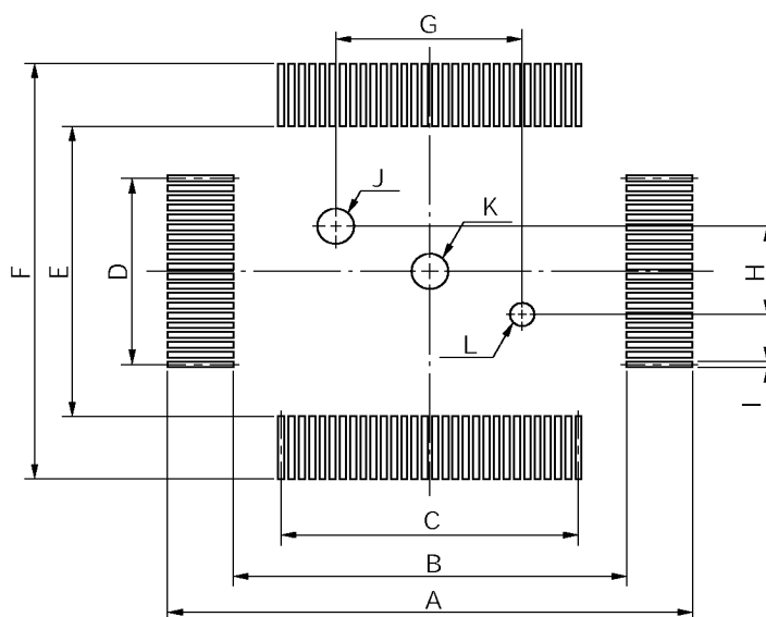
Figure A-2. EV-9200GF-100 Board Mounting Pattern
