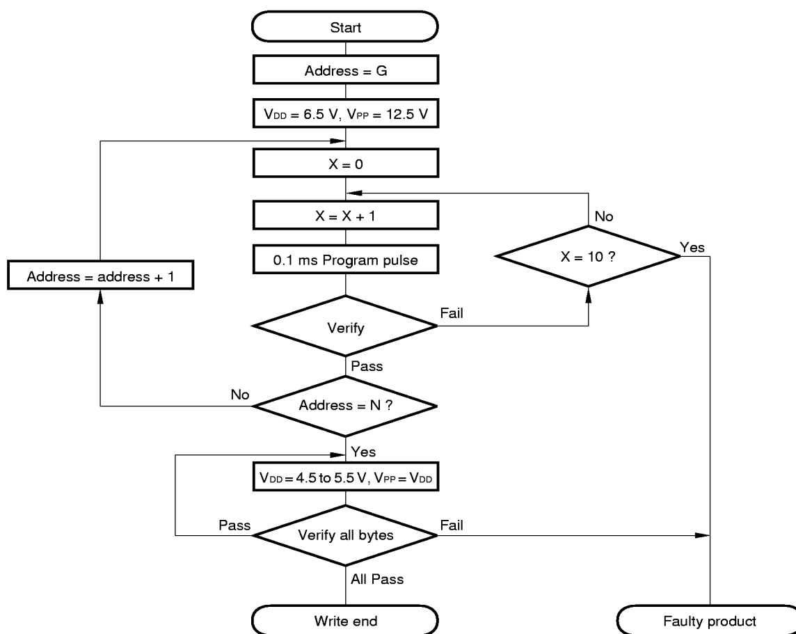
Figure 4-3. Byte Program Mode Flow Chart
