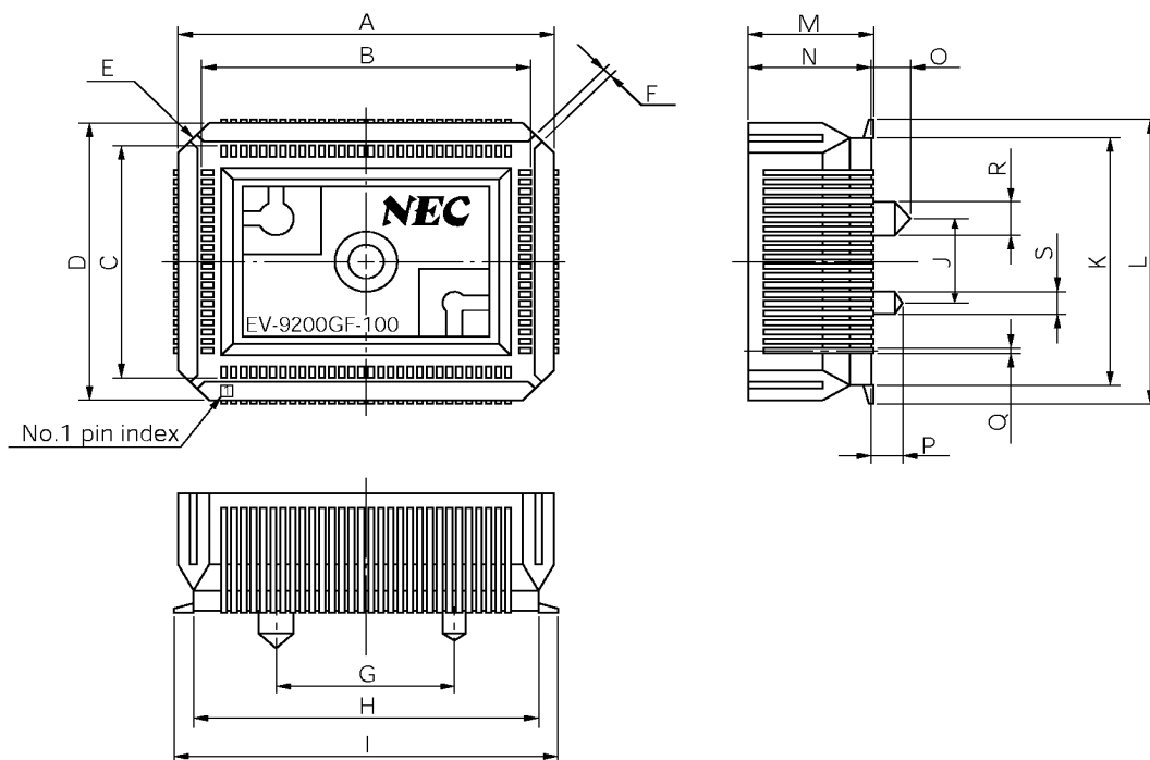
Figure A-1. EV-9200GF-100 Package Drawing
