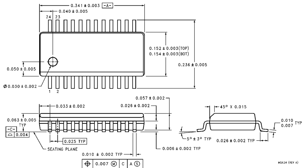
24-Lead Quarter Size Outline Package (QSOP), JEDEC MO-37, 0.150" Wide Package Number MQA24
