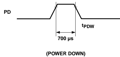
Figure 14. PD minimum pulse width.
