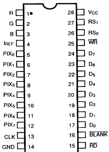
28-PIN DIP
