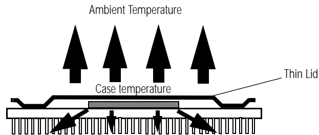
Figure 114. Processor's Heat Dissipation Path
