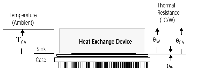
Figure 112. Thermal Model
