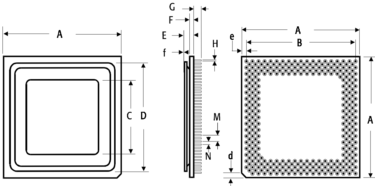
Figure 118. 321-Pin Staggered CPGA Package Specification
