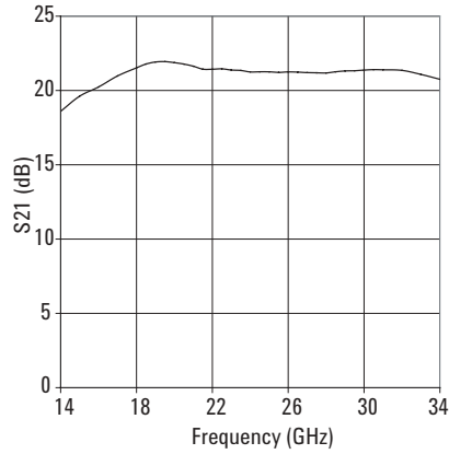
Figure 1. Typical Gain
