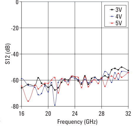
Figure 12: Isolation over Vdd
