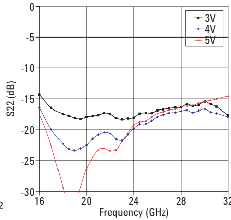
Figure 14: Output Return Loss Over Vdd
