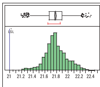
Noise Figure at 26 GHz
