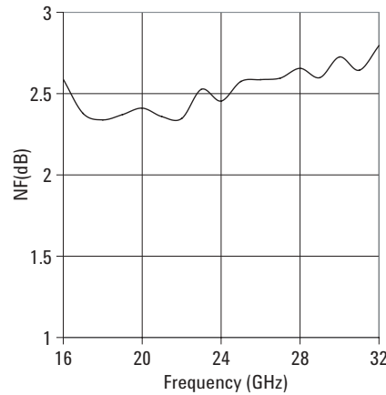
Figure 5. Typical Noise Figure into a 50\ \Omega load.
