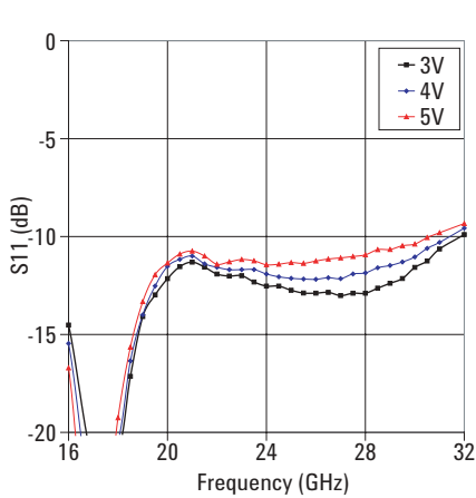
Figure 13: Input Return Loss Over Vdd
