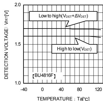
Fig.8 Detecting Voltage Release Voltage
