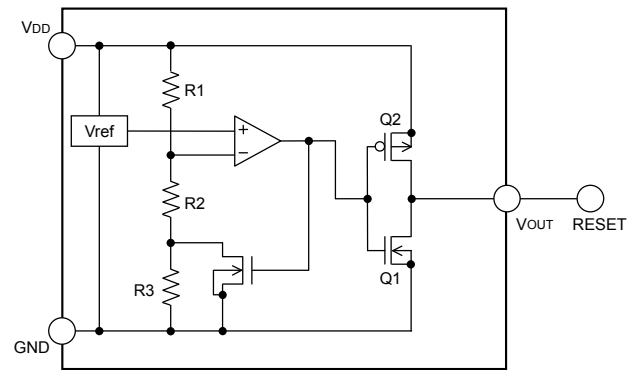
Fig.13 (BU49□□ type internal block diagram)
