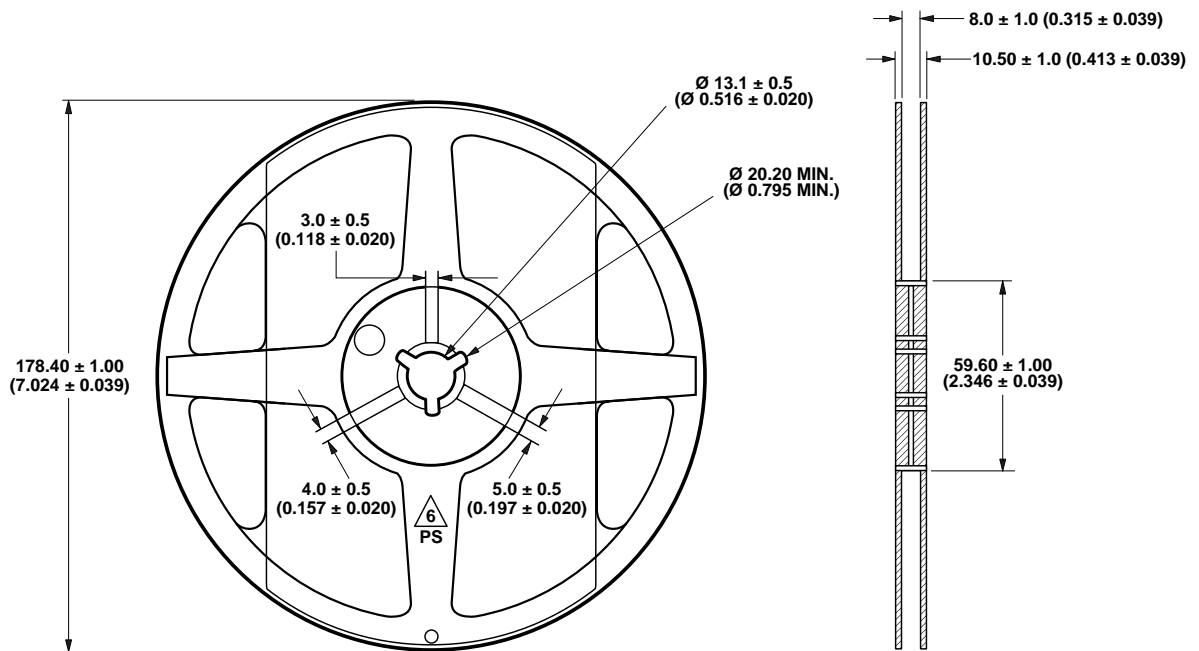
Figure 14. Reel dimensions.
