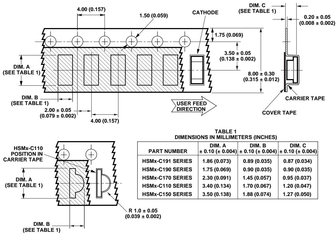
Figure 15. Tape dimensions.
