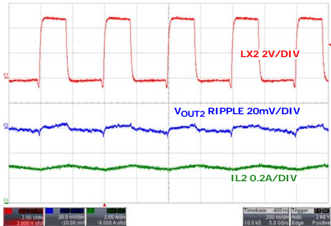
FIGURE 36. STEADY STATE OPERATION WITH FULL LOAD CHANNEL 2
