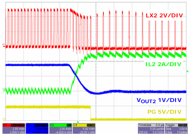
FIGURE 29. OUTPUT SHORT CIRCUIT CHANNEL 2
