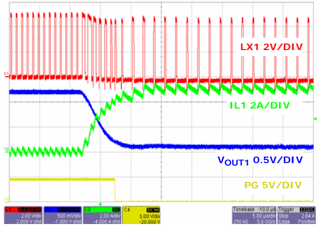
FIGURE 27. OUTPUT SHORT CIRCUIT CHANNEL 1
