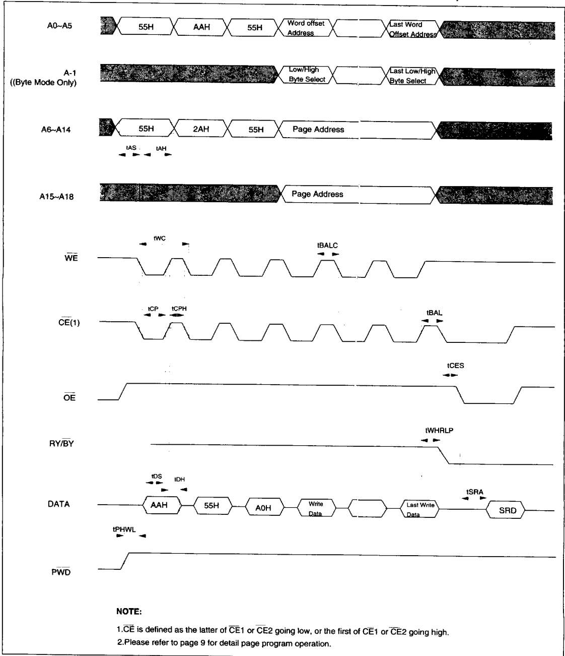
Figure 14. AUTOMATIC PAGE PROGRAM TIMING WAVEFORM(Alternate \overline{CE} Controlled)
