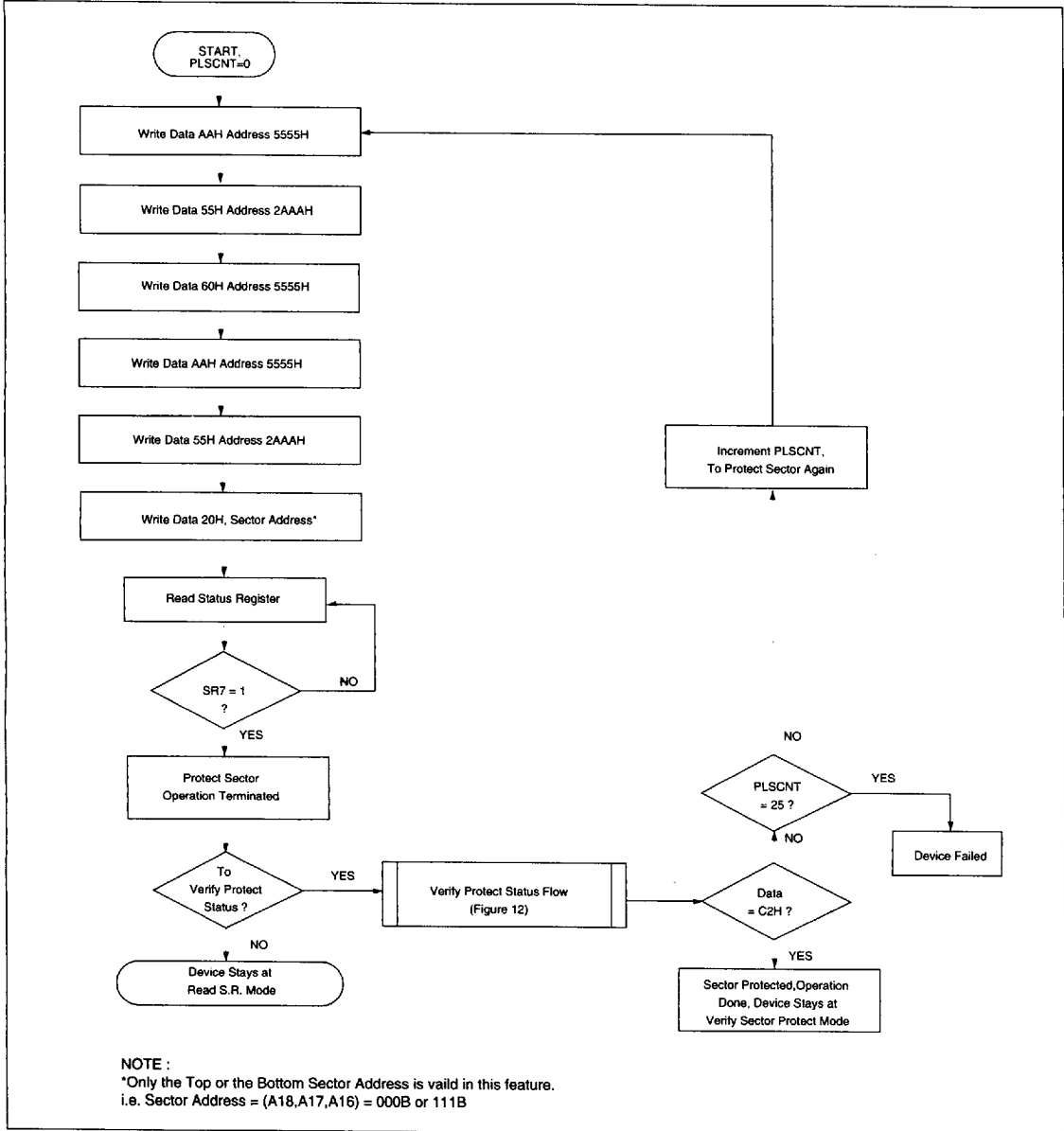
Figure 10. SECTOR PROTECTION ALGORITHM
