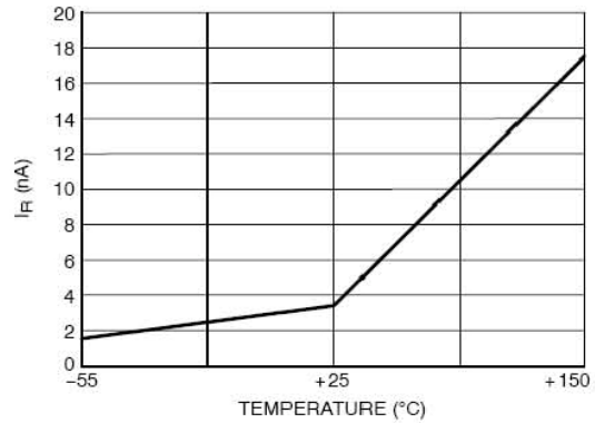
Fig 2. Typical Leakage Current versus Temperature
