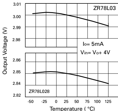
Output Voltage Temperature Coefficient
