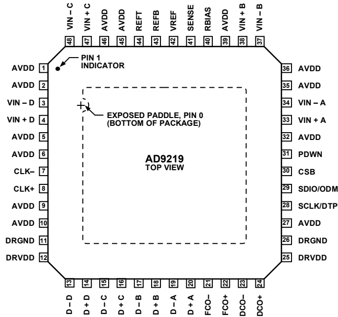
Figure 5. 48-Lead LFCSP Top View
