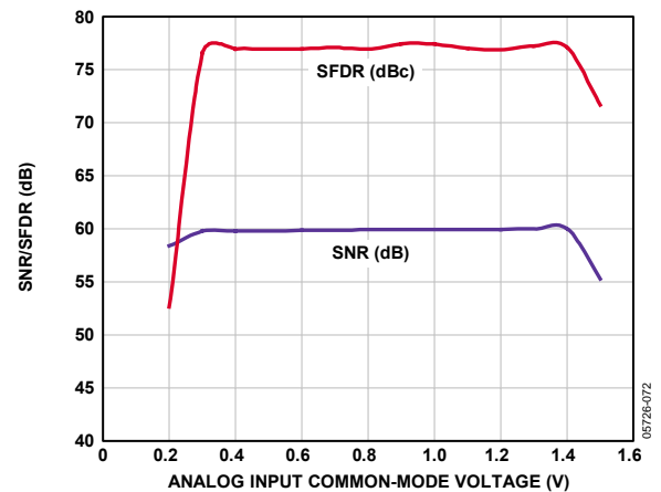
Figure 44. SNR/SFDR vs. Common-Mode Voltage, f_{IN} = 2.4 \text{ MHz} , f_{SAMPLE} = 65 \text{ MSPS}
