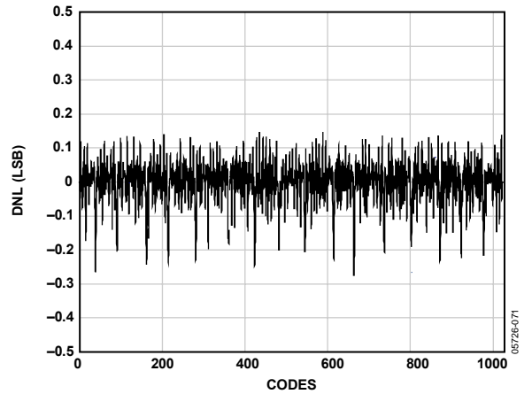
Figure 38. DNL, f_{IN} = 2.4 MHz, f_{SAMPLE} = 65 MSPS
