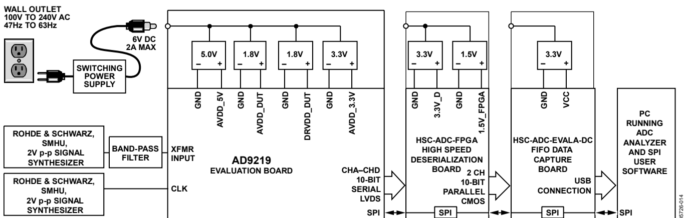
Figure 70. Evaluation Board Connection
