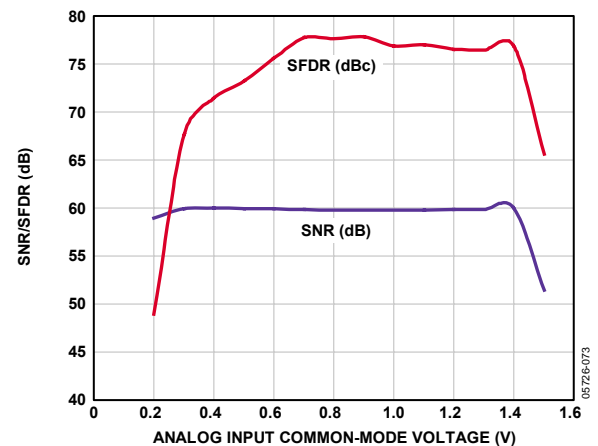
Figure 45. SNR/SFDR vs. Common-Mode Voltage, f_{IN} = 30 \text{ MHz} , f_{SAMPLE} = 65 \text{ MSPS}
