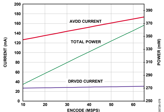
Figure 57. Supply Current vs. f_{\text{SAMPLE}} for f_{\text{IN}} = 10.3 \text{ MHz} , f_{\text{SAMPLE}} = 65 \text{ MSPS}
