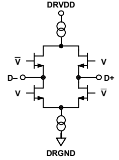
Figure 9. Equivalent Digital Output Circuit
