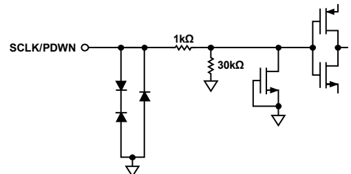
Figure 10. Equivalent SCLK/PDWN Input Circuit
