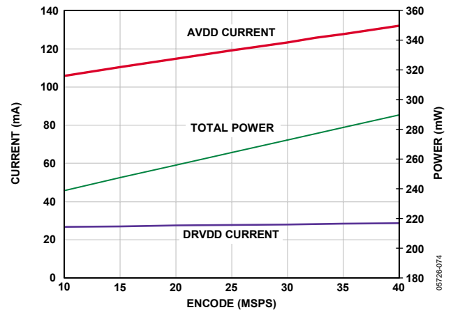
Figure 56. Supply Current vs. f_{\text{SAMPLE}} for f_{\text{IN}} = 10.3 \text{ MHz} , f_{\text{SAMPLE}} = 40 \text{ MSPS}
