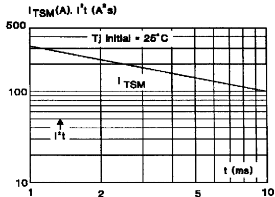
Fig.8 : Non repetitive surge peak on-state current for a sinusoidal pulse with width : t \leq 10\text{ms} , and corresponding value of I^2t .
