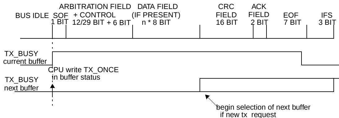
Figure 64. Data Transmission
