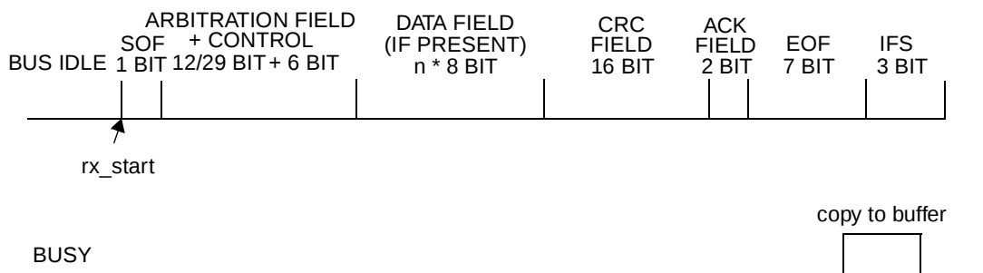
Figure 61. Receive Timing
