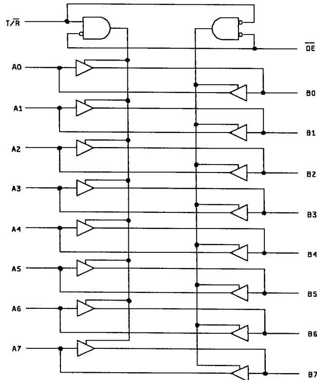
FIGURE 3. Logic diagram.
