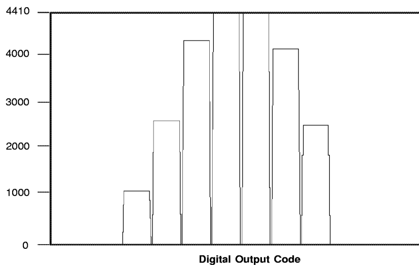
Figure 7. ADS-932 Grounded Input Histogram
