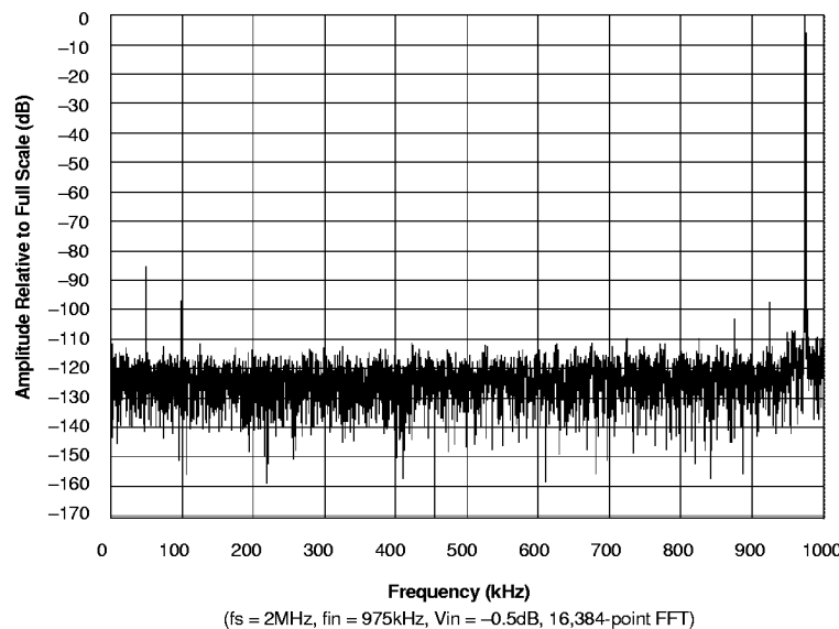
Figure 4. FFT Analysis of ADS-932
