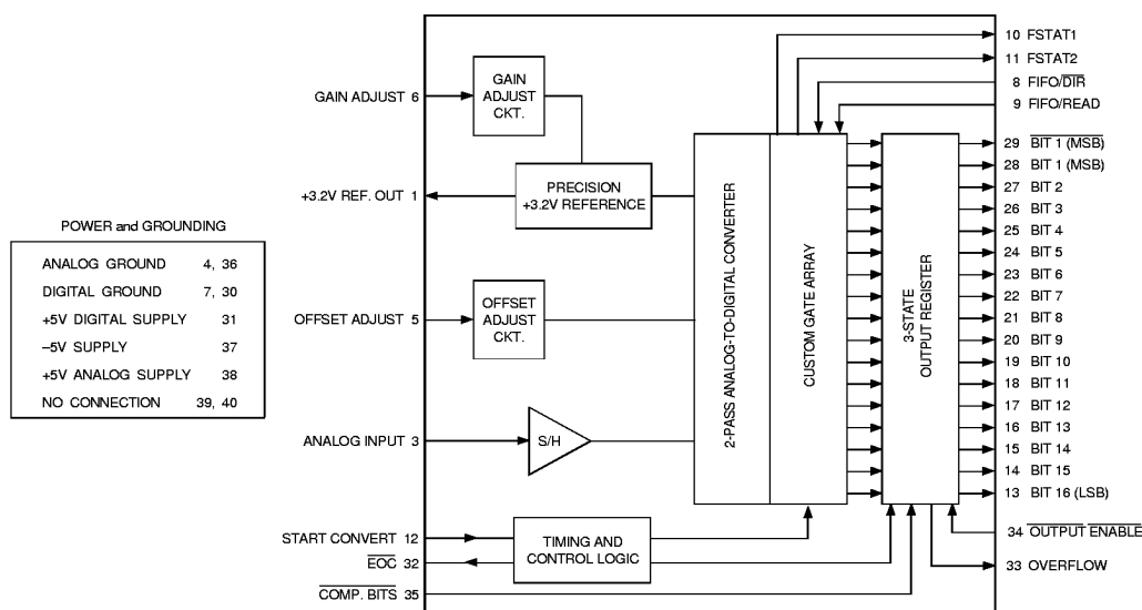
Figure 1. ADS-932 Functional Block Diagram
