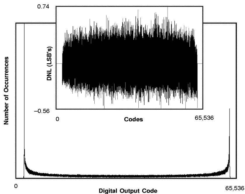
Figure 6. ADS-932 Histogram and Differential Nonlinearity
