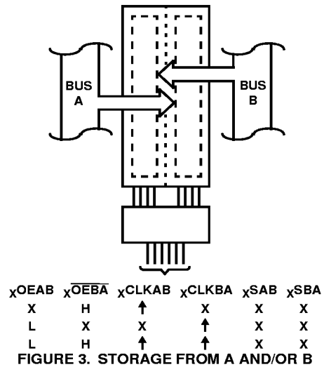
FIGURE 3. STORAGE FROM A AND/OR B
