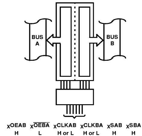
FIGURE 4. TRANSFER STORES DATA TO A AND/OR B
