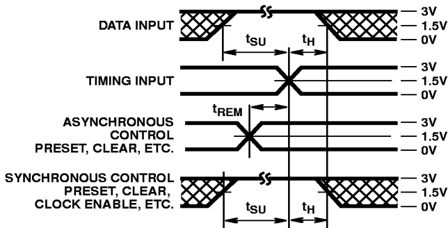
FIGURE 6. SETUP, HOLD, AND RELEASE TIMING
