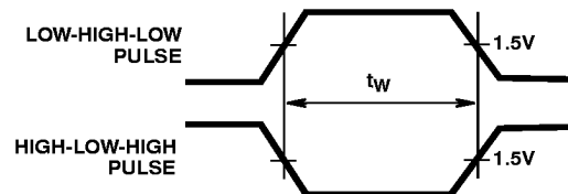
FIGURE 7. PULSE WIDTH
