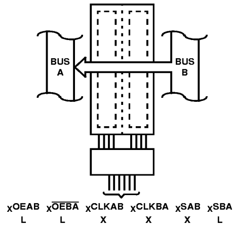
FIGURE 1. REAL-TIME TRANSFER BUS B TO A
