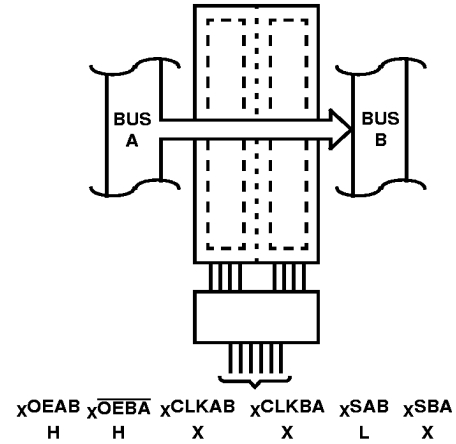
FIGURE 2. REAL-TIME TRANSFER BUS A TO B
