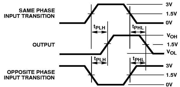
FIGURE 9. PROPAGATION DELAY
