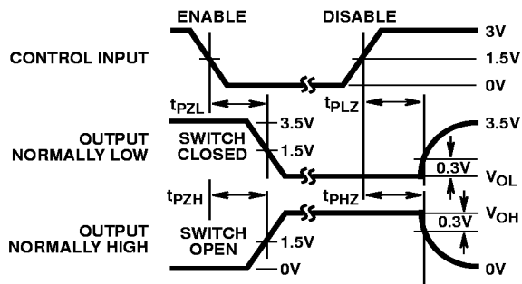
FIGURE 8. ENABLE AND DISABLE TIMING
