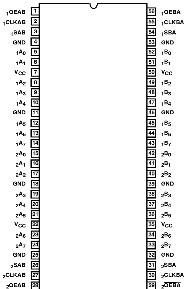
CD74FCT16652T, CD74FCT162652T (SSOP, TSSOP) TOP VIEW
