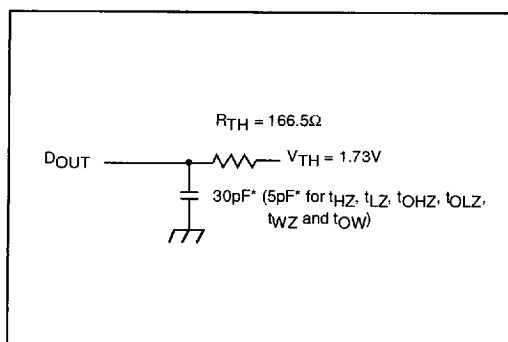
Figure 2. Thevenin Equivalent
