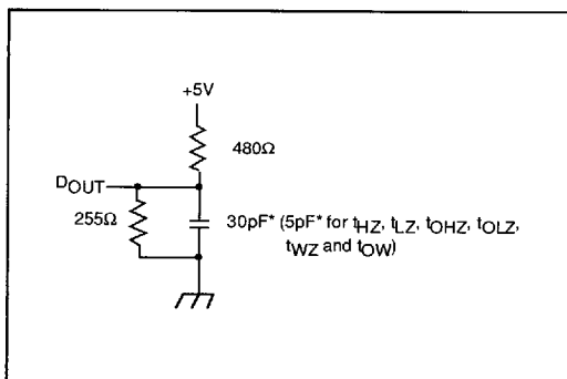
Figure 1. Output Load
