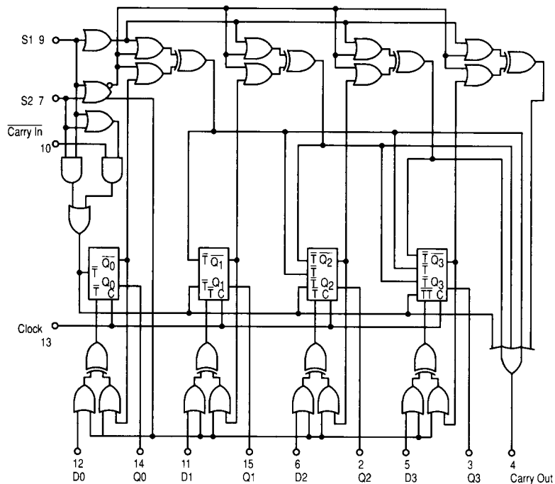
Figure 1. Logic Diagram
