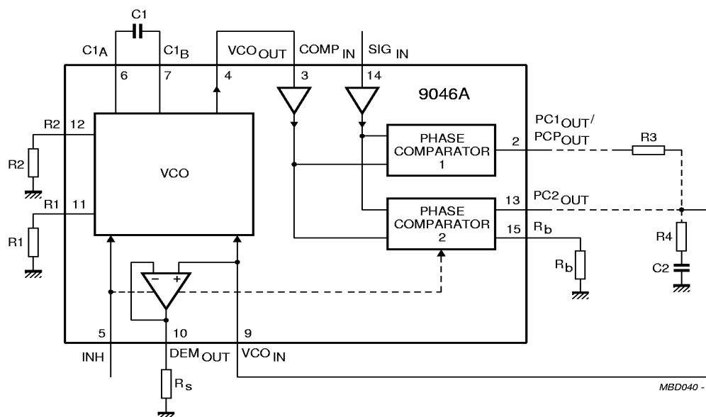
Fig.4 Functional diagram.
