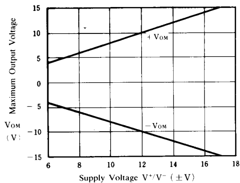
Maximum Output Voltage Swing vs. Supply Voltage
