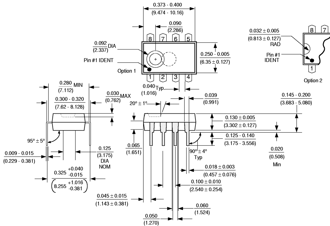
Molded Dual-In-Line Package (N) Package Number N08E
