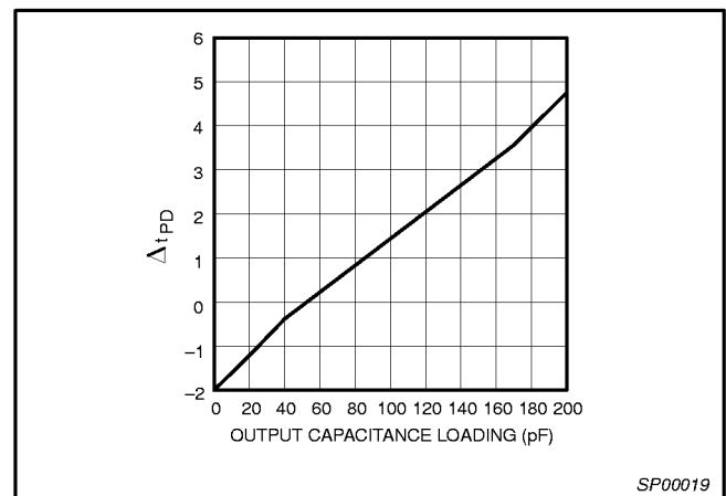
Figure 2. \Delta t_{\text{PD}} vs Output Capacitance Loading (Typical)
