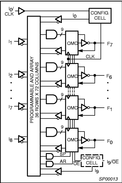
FUNCTIONAL DIAGRAM
