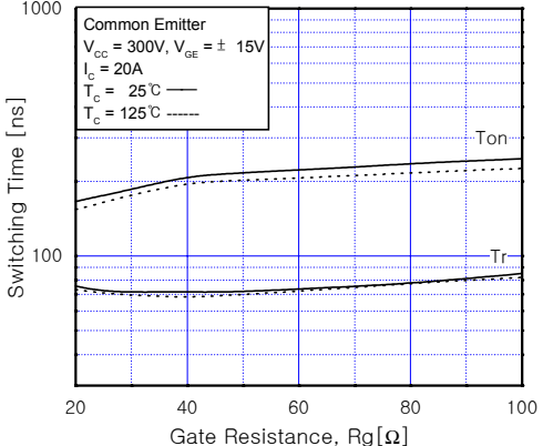
Fig 7. Turn-On Characteristics vs. Gate Resistance
