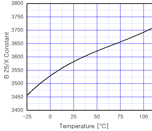
Fig 20. NTC Characteristics
