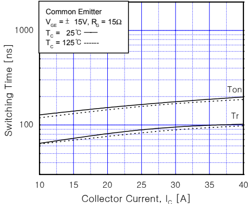
Fig 10. Turn-On Characteristics vs. Collector Current
