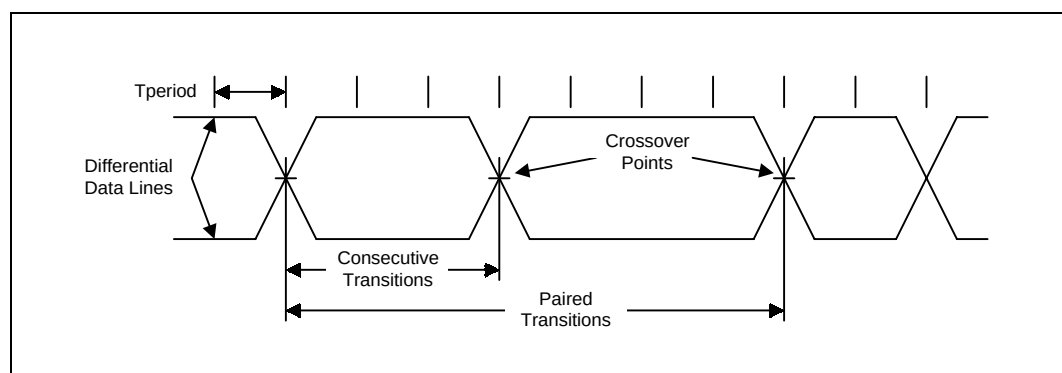
Figure 14-14. USB Jitter
