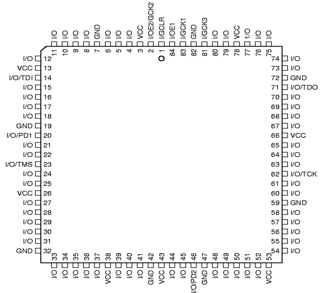
84-Lead PLCC Top View
