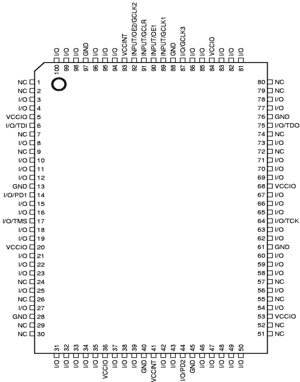
100-Lead PQFP Top View
