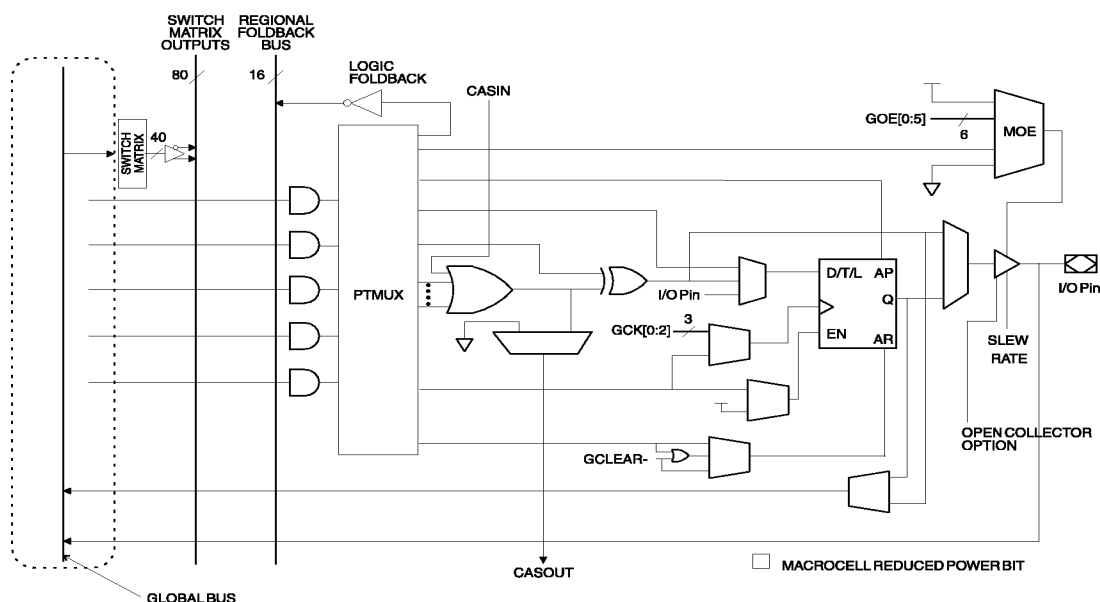
Figure 1. ATF1504AS Macrocell
