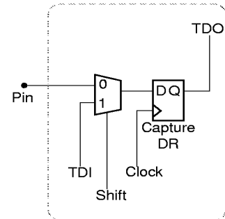
Pin BSC
