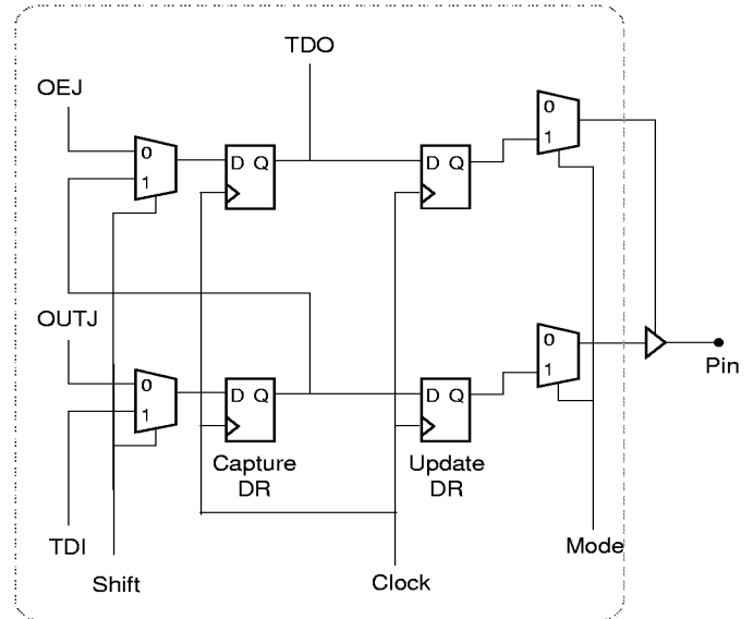
Macrocell BSC
