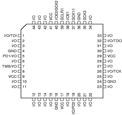
44-Lead TQFP Top View
