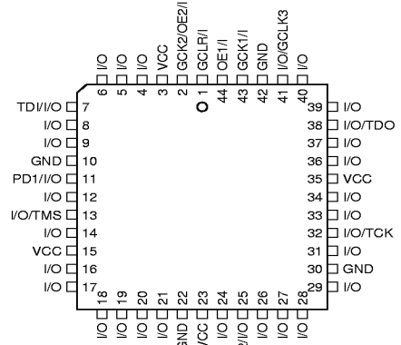
44-Lead PLCC Top View
