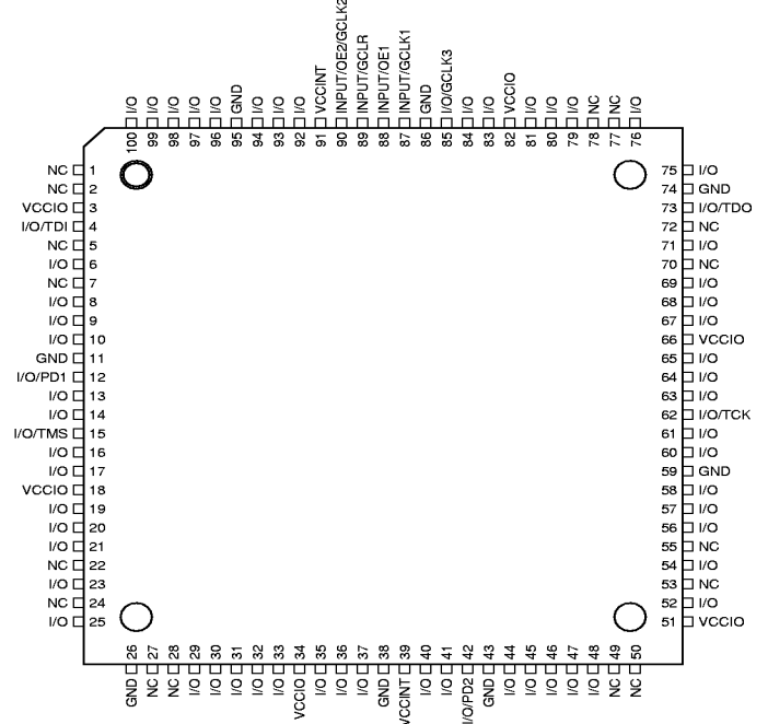
100-Lead TQFP Top View
