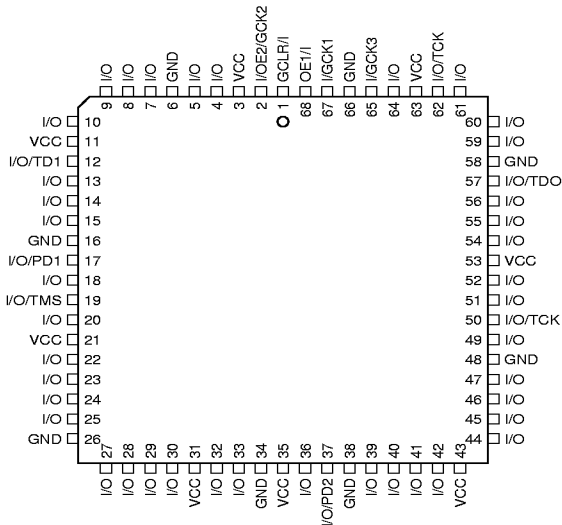
68-Lead PLCC Top View
