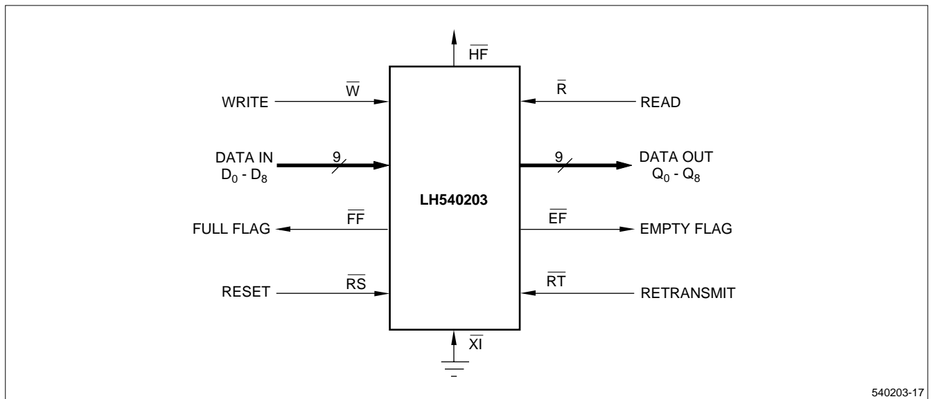
Figure 4. Standalone FIFO (2048 × 9)
