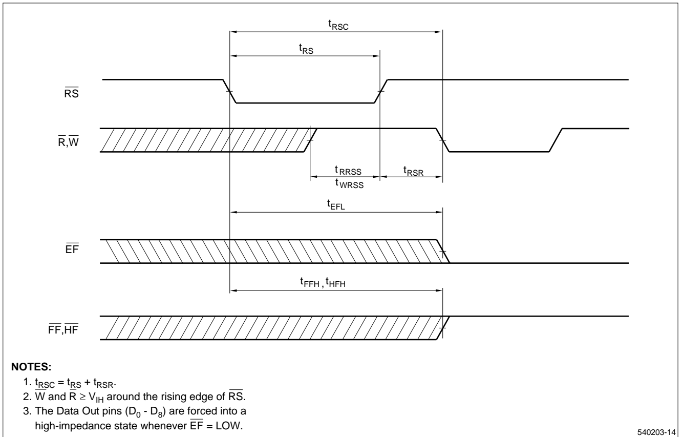
Figure 10. Reset Timing
