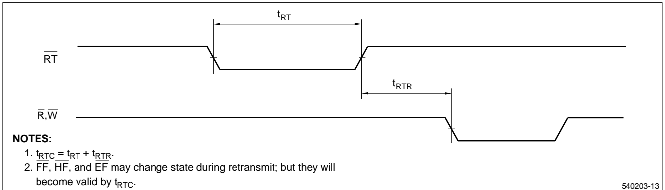
Figure 19. Retransmit Timing
