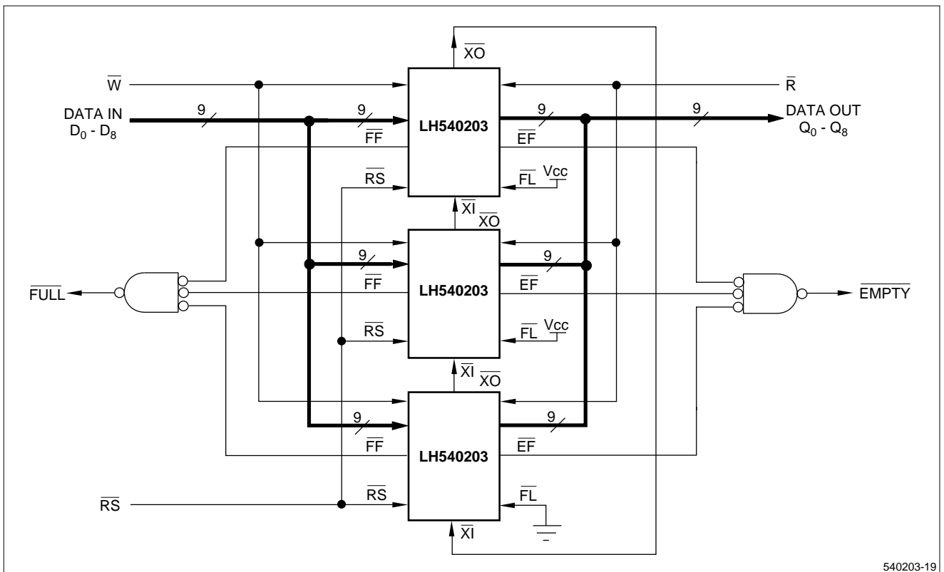
Figure 6. FIFO Depth Cascading (6144 × 9)
