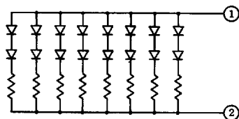
Internal connection diagram
