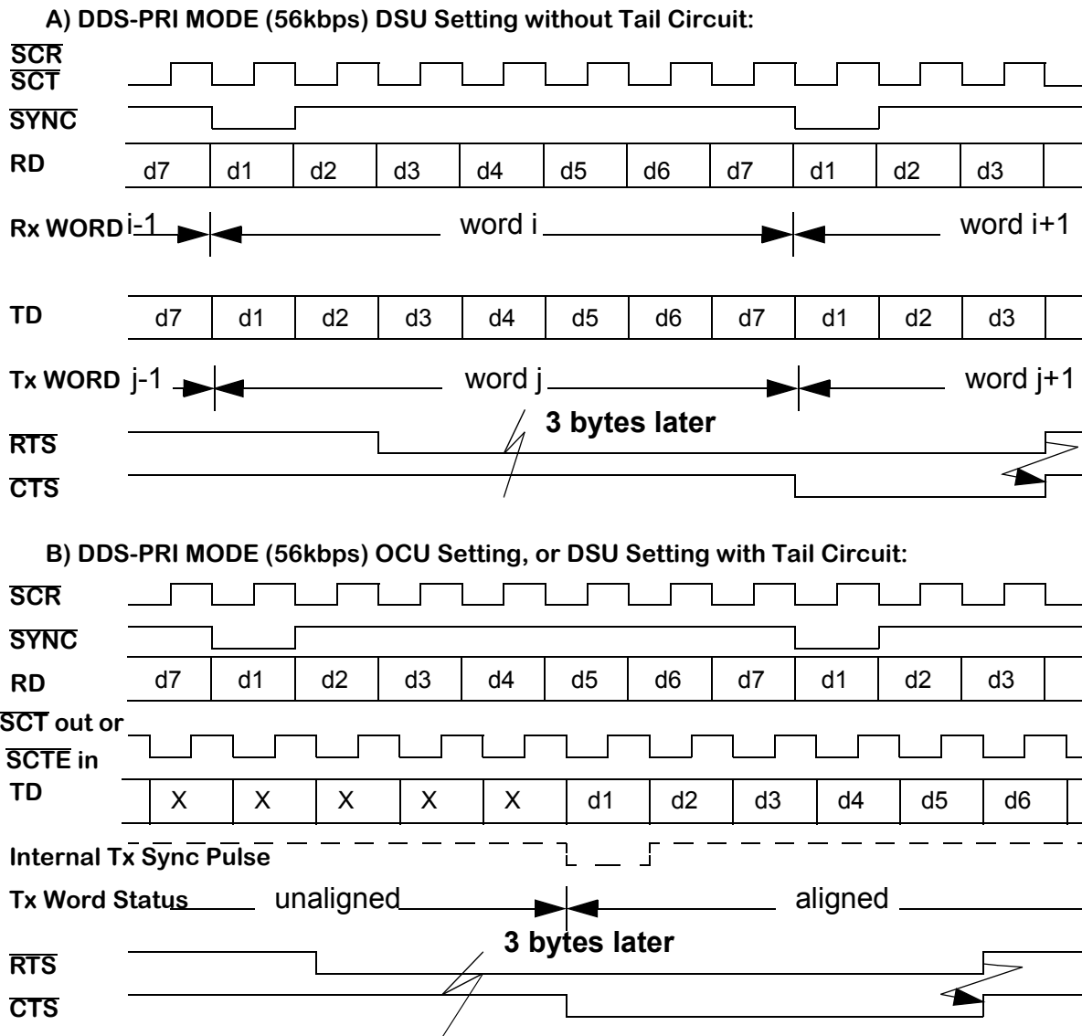
Figure 6: EIA Interface Data Structure & Timing - DDS-PRI Mode
