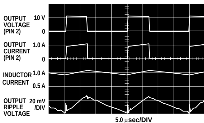
Figure 30. Switching Waveforms
