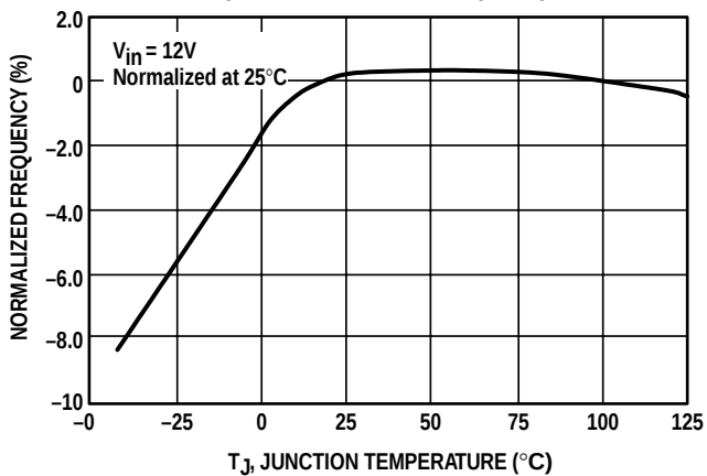
Figure 28. Oscillator Frequency
