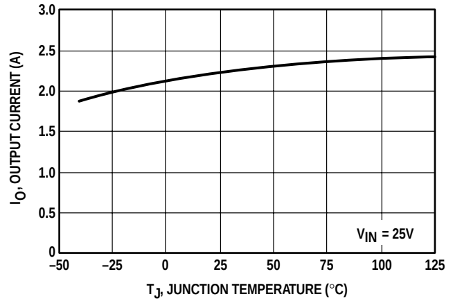
Figure 23. Current Limit
