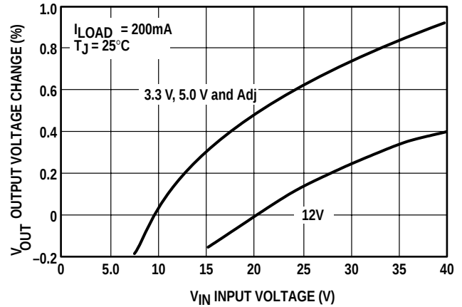
Figure 21. Line Regulation
