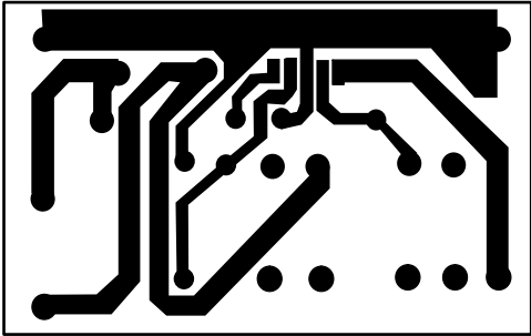
Figure 19. PC Board Copper Side
