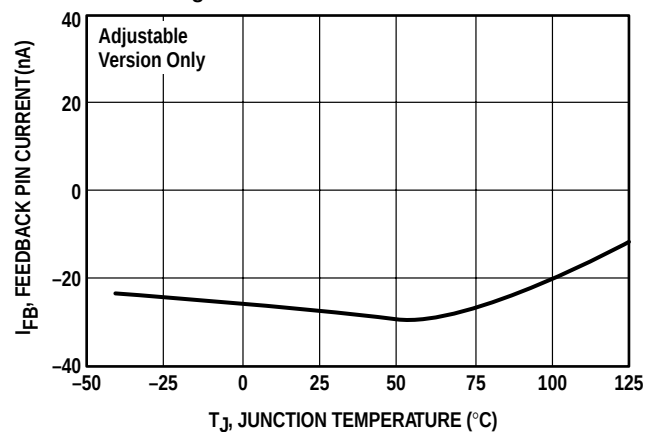
Figure 29. Feedback Pin Current
