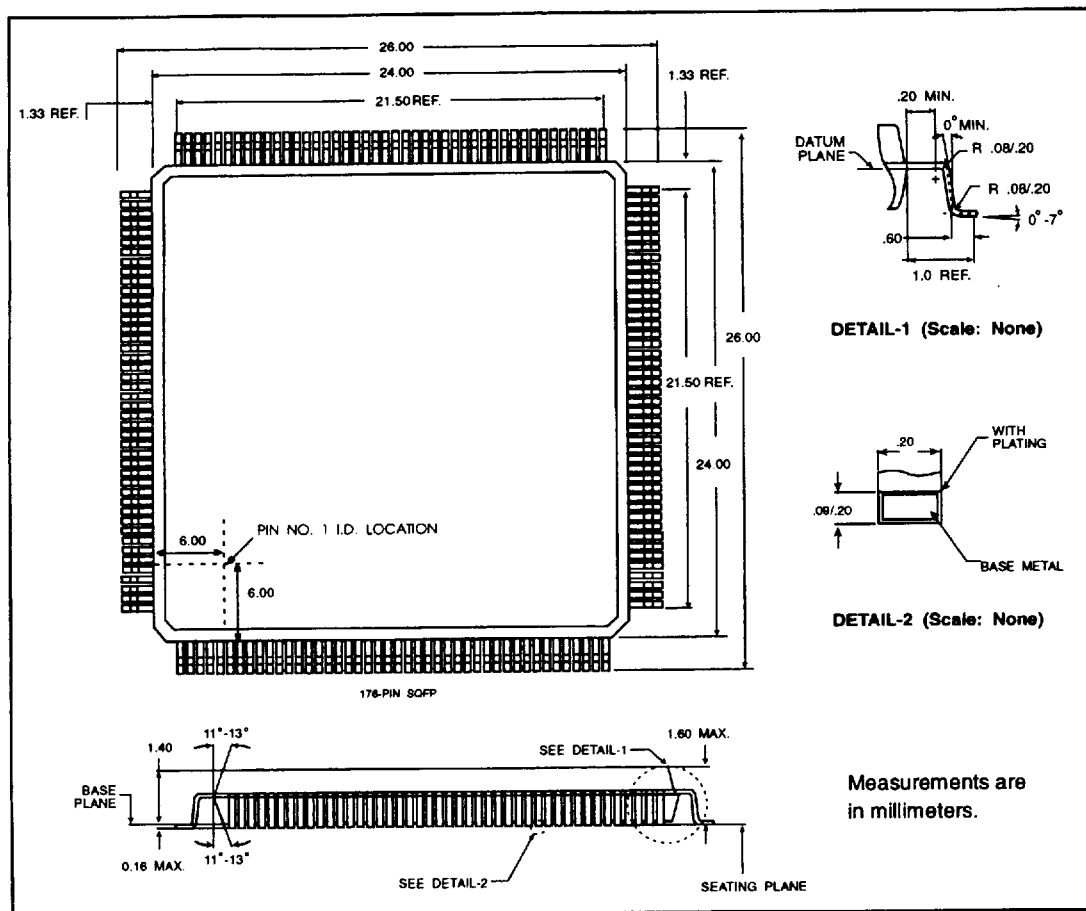
FIGURE 8-1 176-PIN SQFP
