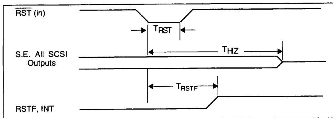
FIGURE 7-28 SCSI RESET
