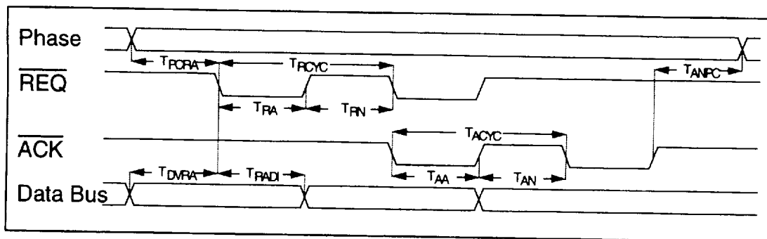
FIGURE 7-23 TARGET SYNCHRONOUS IN
