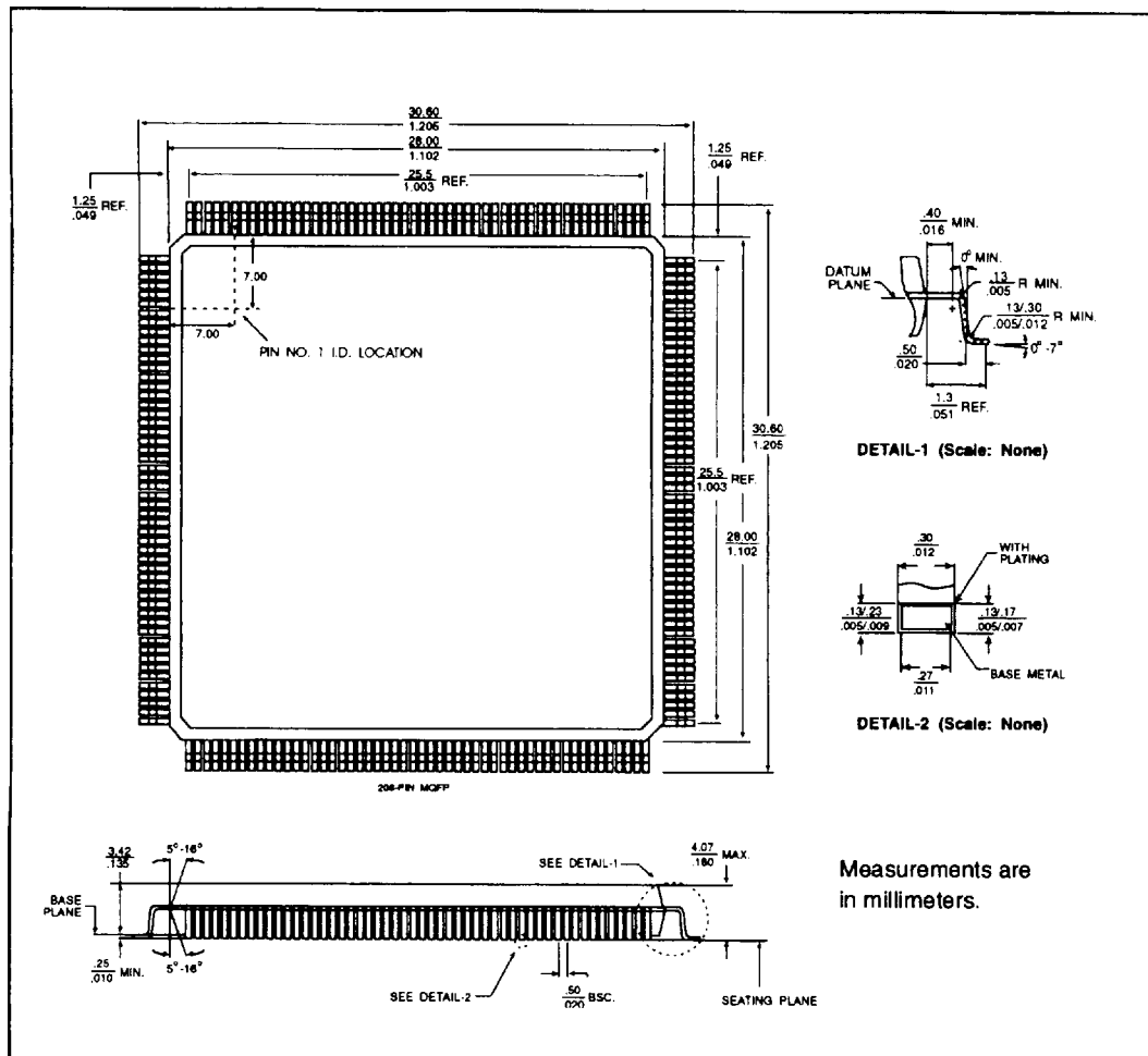
FIGURE 8-2 208-PIN MQFP
