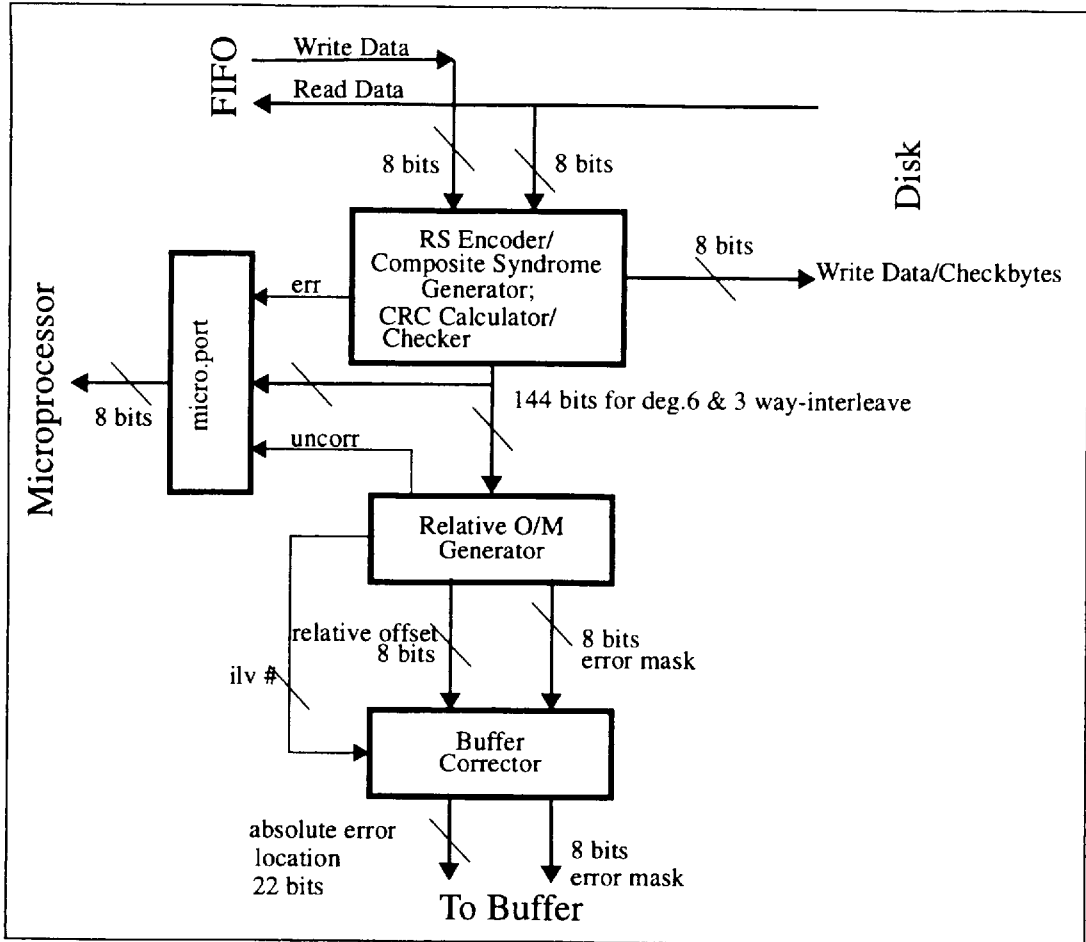
FIGURE 5-21 ECC ARCHITECTURE
