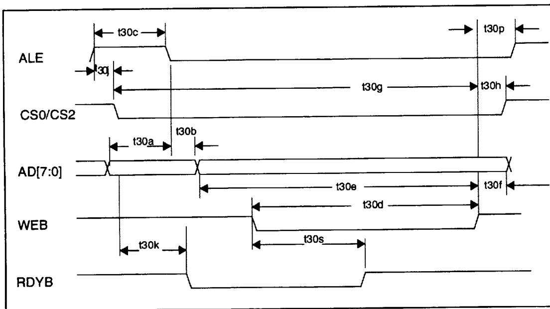
FIGURE 7-4 PIO WRITE WITH RDYB - BUFFER ACCESS
