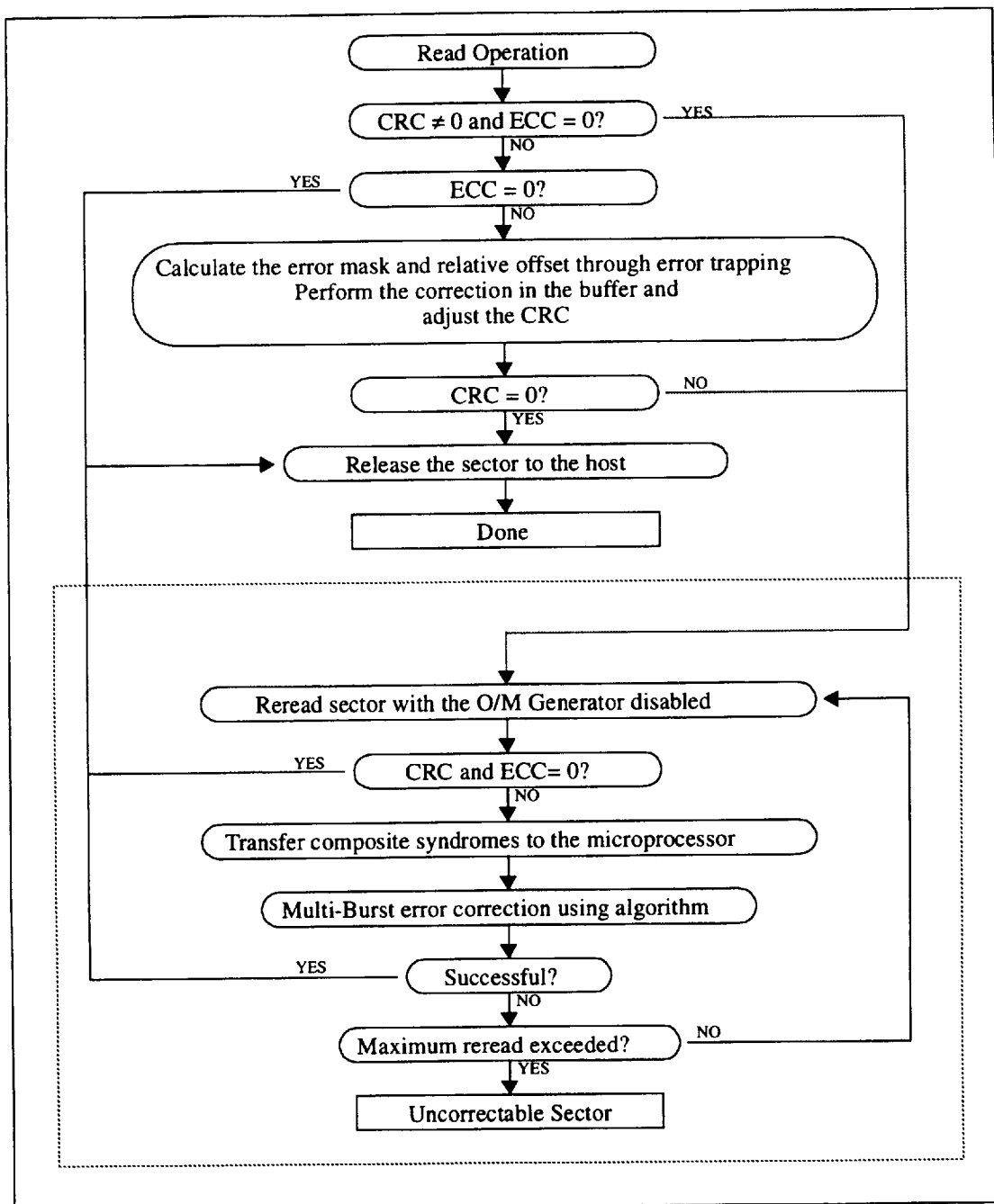
FIGURE 5-23 MICROPROCESSOR CONTROL
