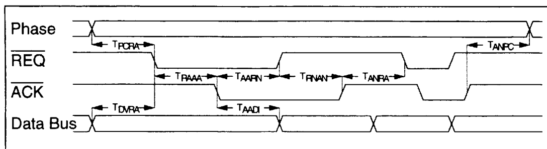
FIGURE 7-20 TARGET ASYNCHRONOUS IN
