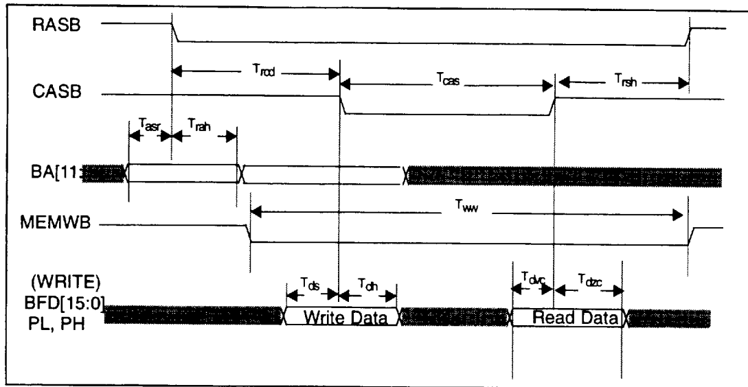
FIGURE 7-10 DMA Read/Write RAS/CAS TIMING
