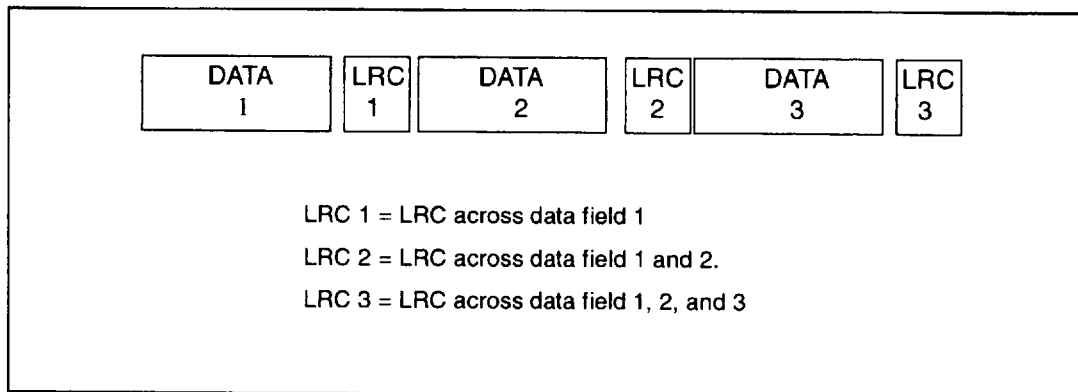
FIGURE 5-25 LRC EXAMPLE
