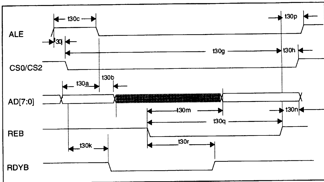
FIGURE 7-3 PIO READ WITH RDYB - BUFFER ACCESS
