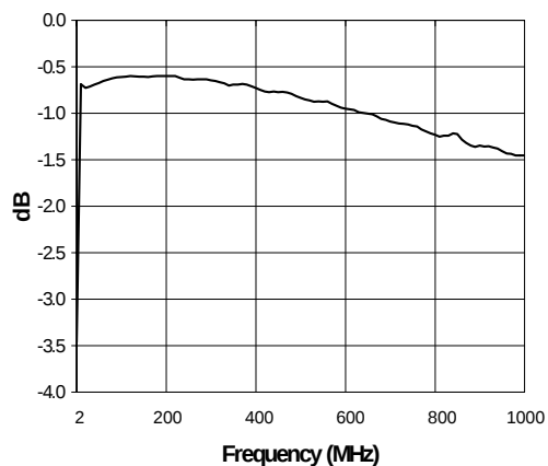
Insertion Loss
