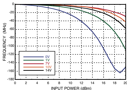
Fcenter vs. Input Power
