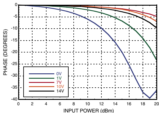
Insertion Phase vs. Input Power
