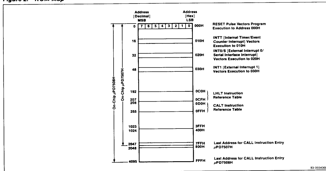
Figure 2. ROM Map
