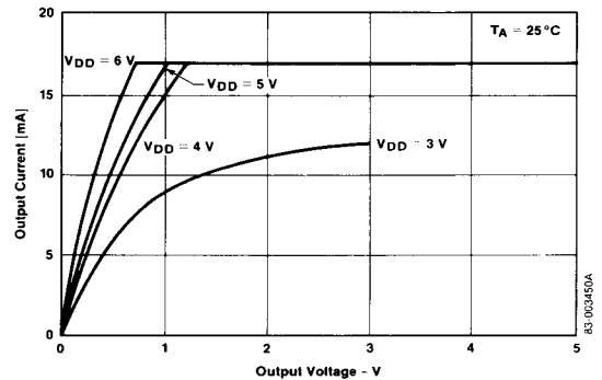
V_{OL} vs. I_{OL} [Ports 2-7]
