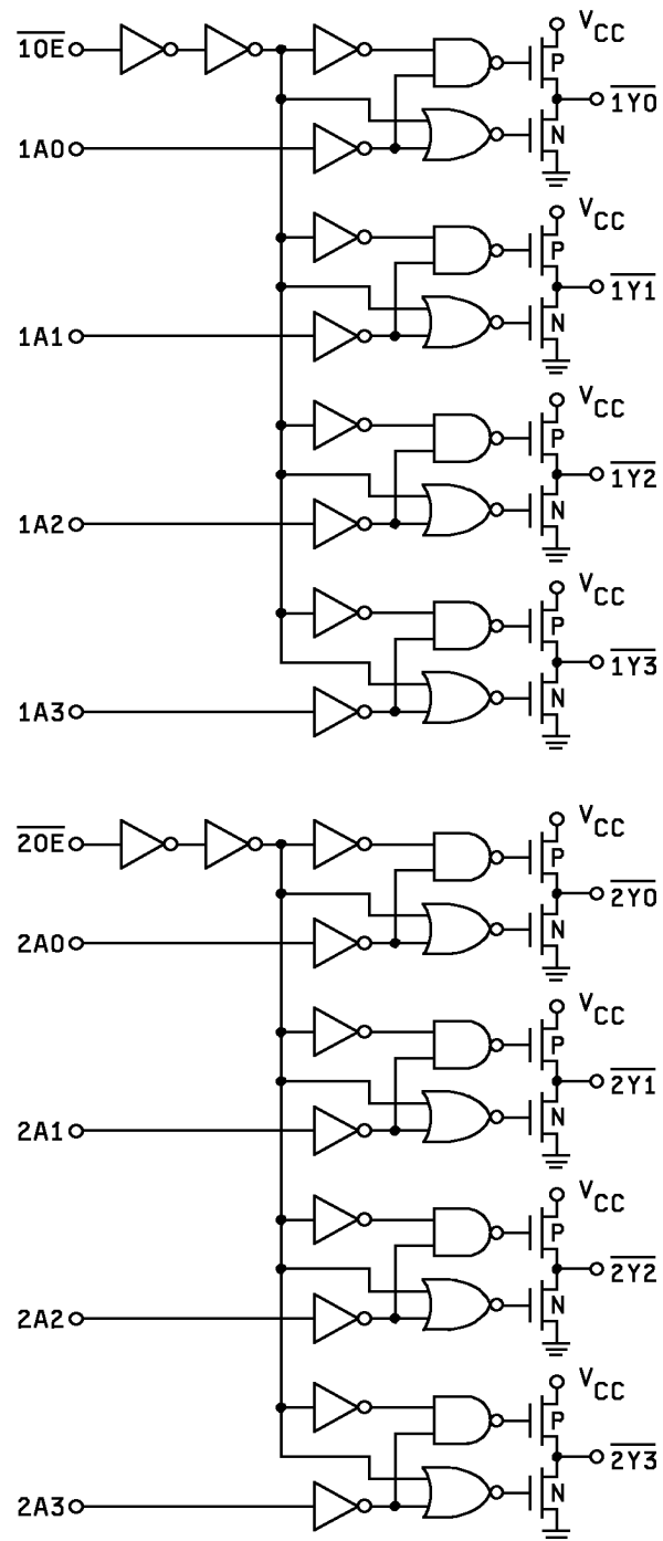
FIGURE 3. Logic diagram.
