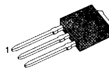
1.Gate 2.Drain 3.Source IRFU420/421
