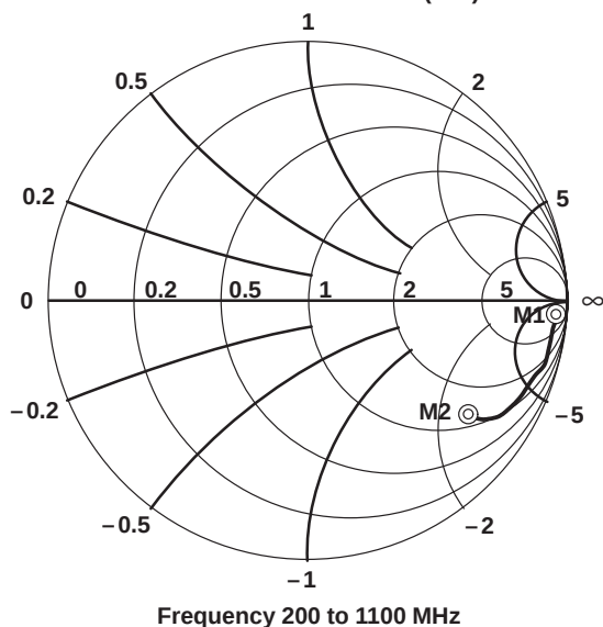
Mixer IF Output (MIX_OUT–, MIX_OUT+) Differential 1-Port S-Parameter (S11)
