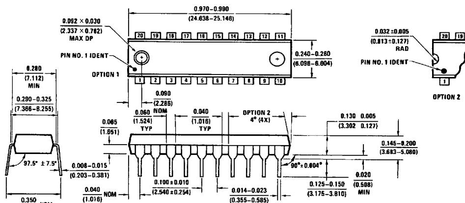
20-Lead Molded Thin Shrink Small Outline Package, JEDEC NS Package Number MTC20
