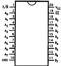
Pin Assignment for DIP, Flatpak, SSOP and SOIC
