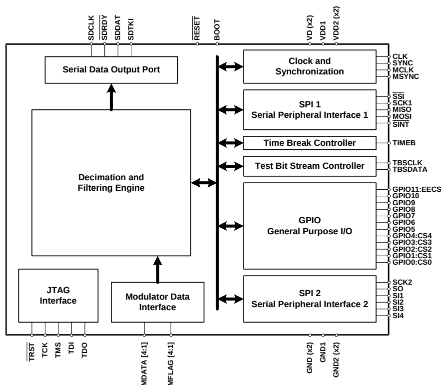
Figure 1. CS5376A Block Diagram
