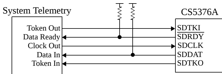
Figure 31. Serial Data Port Block Diagram
