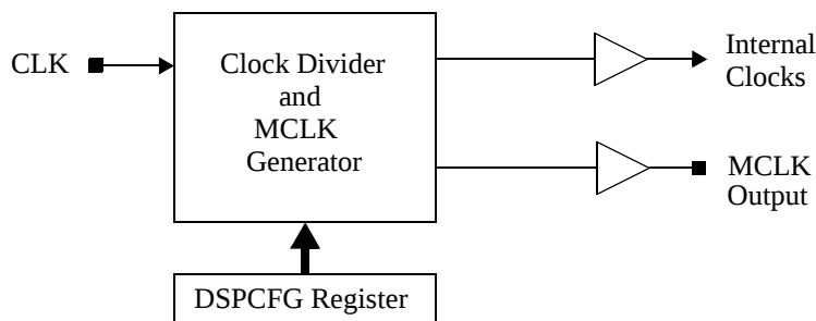
Figure 12. Clock Generation Block Diagram
