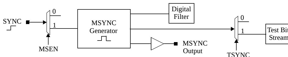
Figure 13. Synchronization Block Diagram
