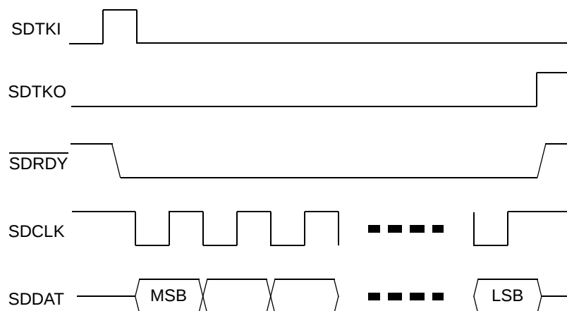
Figure 33. SD Port Transaction
